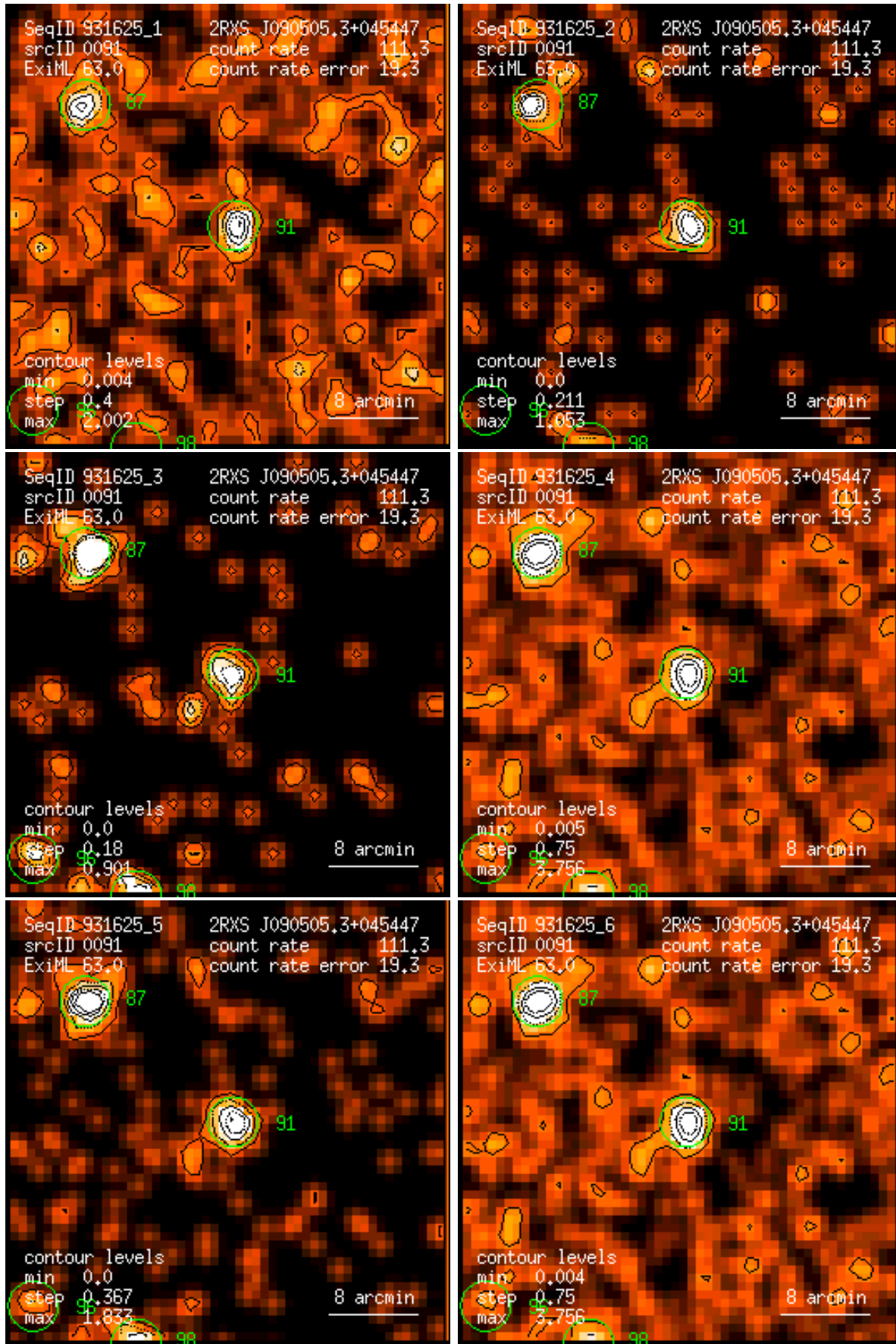
Figure 91: RASS 931625: detection 0091: band rate images, Gaussian filter: (1) PSPC channels 11 – 41, (2) 52 – 90, (3) 91 – 201, (4) 11 – 235, (5) 52 – 201, (6) 11 – 201. Broad band rates in counts/ks. Band rate contour levels in counts/ks/arcmin 2 .
