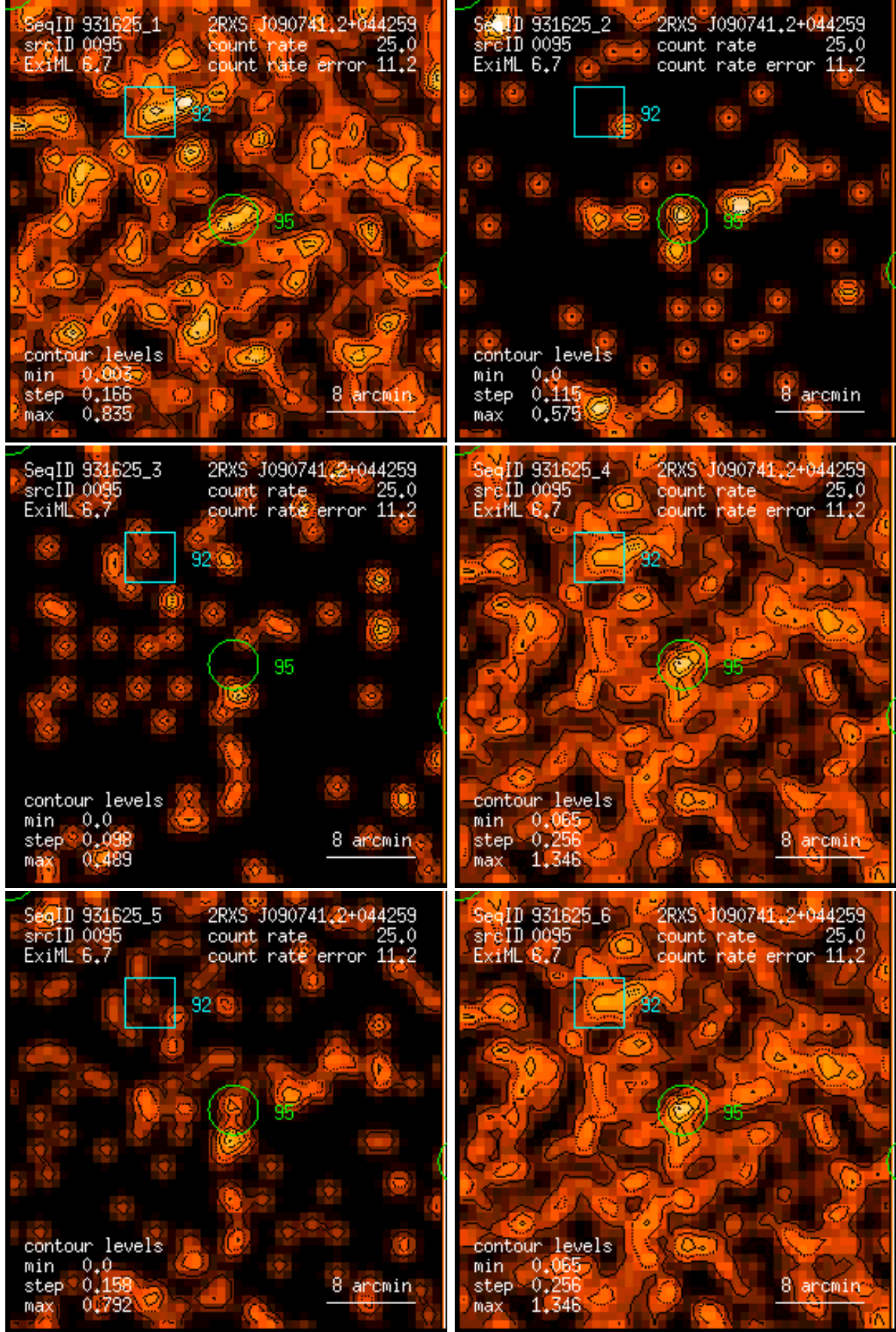
Figure 95: RASS 931625: detection 0095: band rate images, Gaussian filter: (1) PSPC channels 11 – 41, (2) 52 – 90, (3) 91 – 201, (4) 11 – 235, (5) 52 – 201, (6) 11 – 201. Broad band rates in counts/ks. Band rate contour levels in counts/ks/arcmin 2 .
