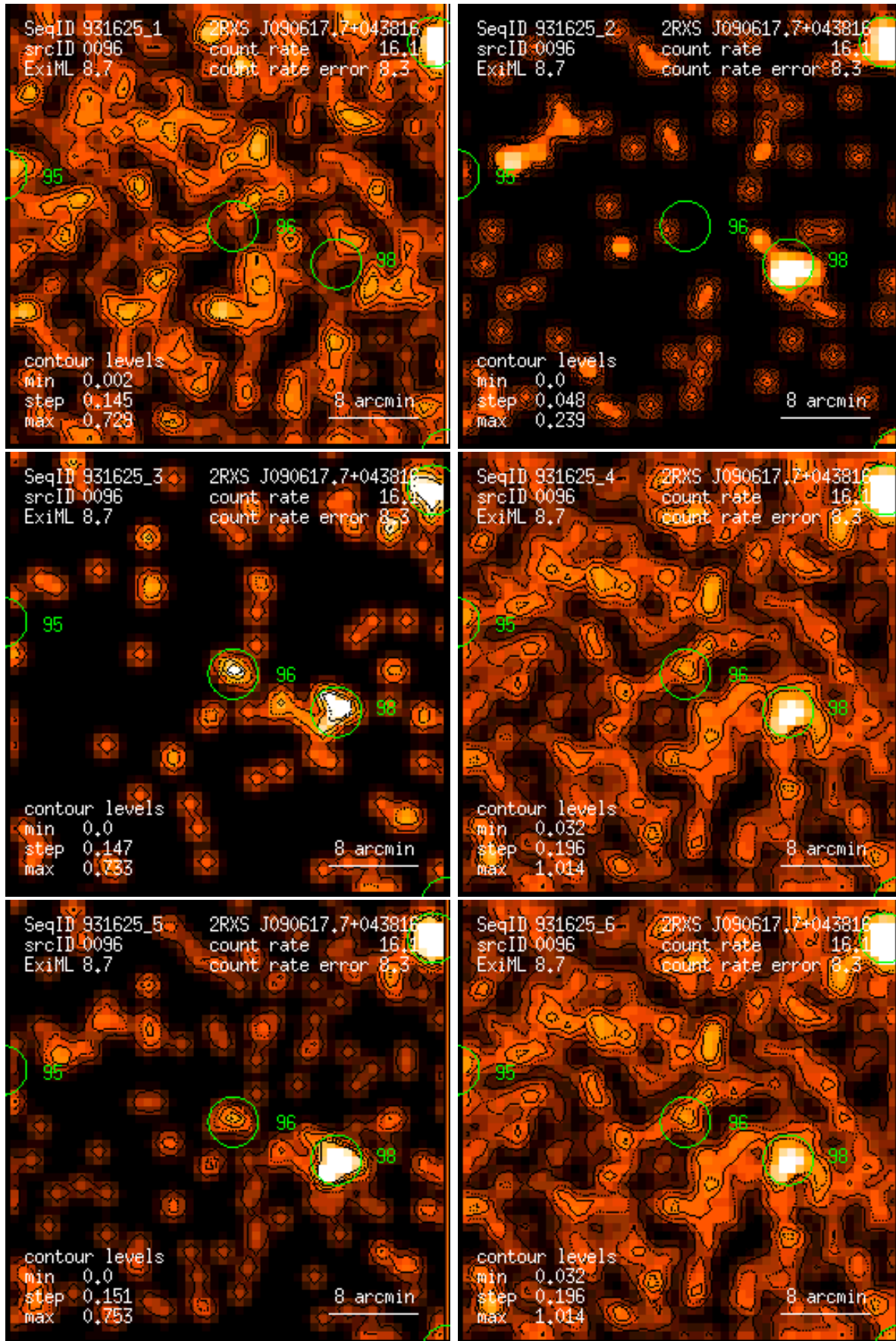
Figure 96: RASS 931625: detection 0096: band rate images, Gaussian filter: (1) PSPC channels 11 – 41, (2) 52 – 90, (3) 91 – 201, (4) 11 – 235, (5) 52 – 201, (6) 11 – 201. Broad band rates in counts/ks. Band rate contour levels in counts/ks/arcmin 2 .
