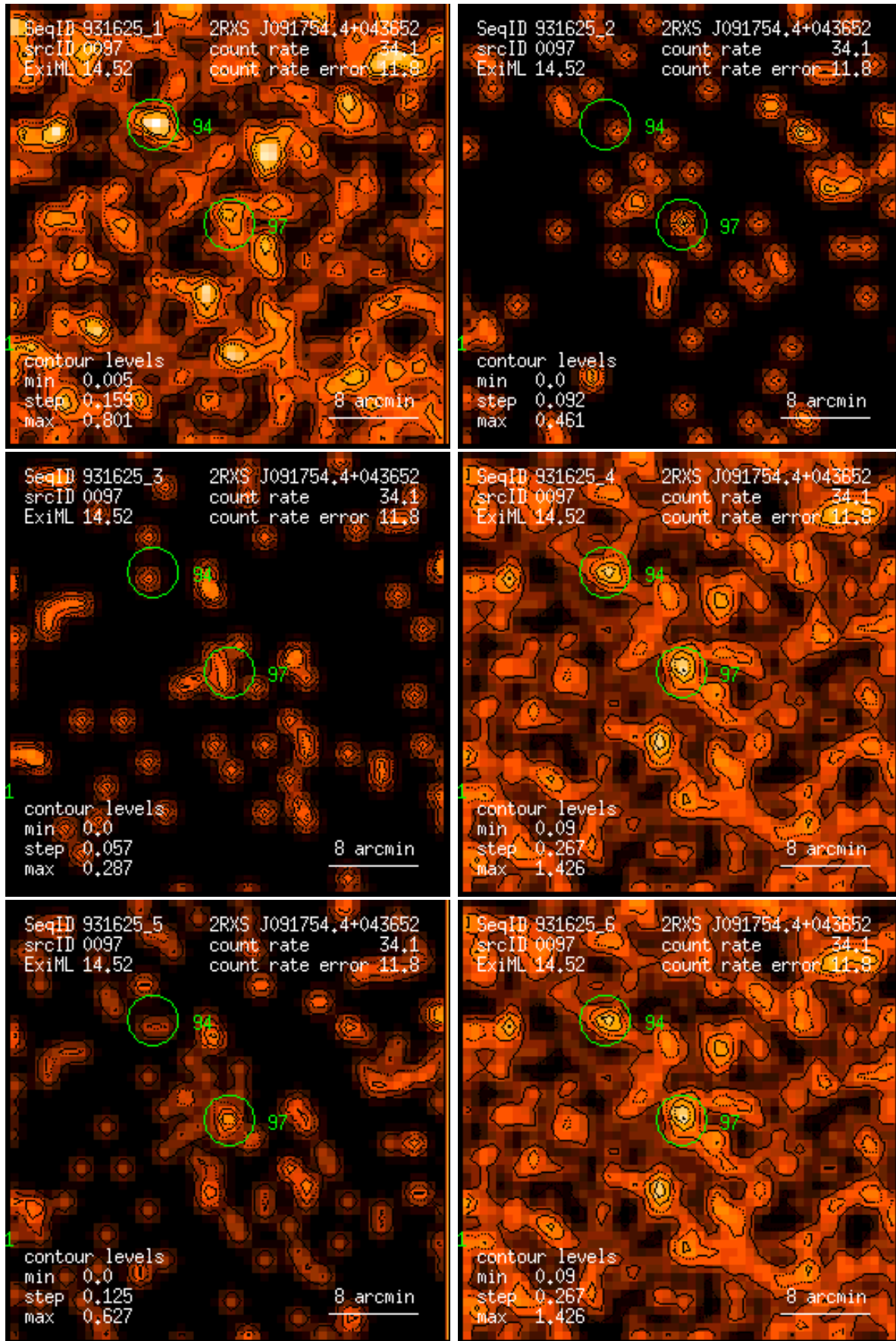
Figure 97: RASS 931625: detection 0097: band rate images, Gaussian filter: (1) PSPC channels 11 – 41, (2) 52 – 90, (3) 91 – 201, (4) 11 – 235, (5) 52 – 201, (6) 11 – 201. Broad band rates in counts/ks. Band rate contour levels in counts/ks/arcmin 2 .
