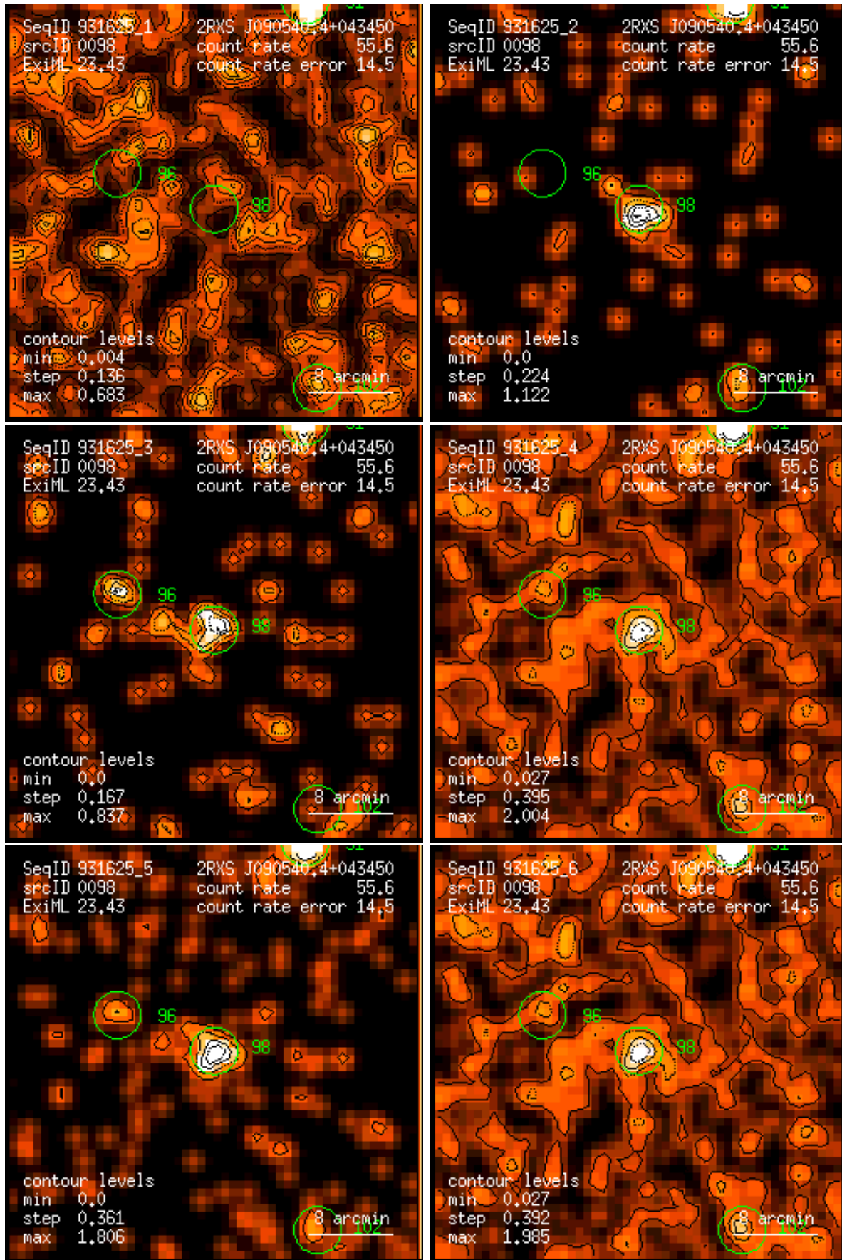
Figure 98: RASS 931625: detection 0098: band rate images, Gaussian filter: (1) PSPC channels 11 – 41, (2) 52 – 90, (3) 91 – 201, (4) 11 – 235, (5) 52 – 201, (6) 11 – 201. Broad band rates in counts/ks. Band rate contour levels in counts/ks/arcmin 2 .
