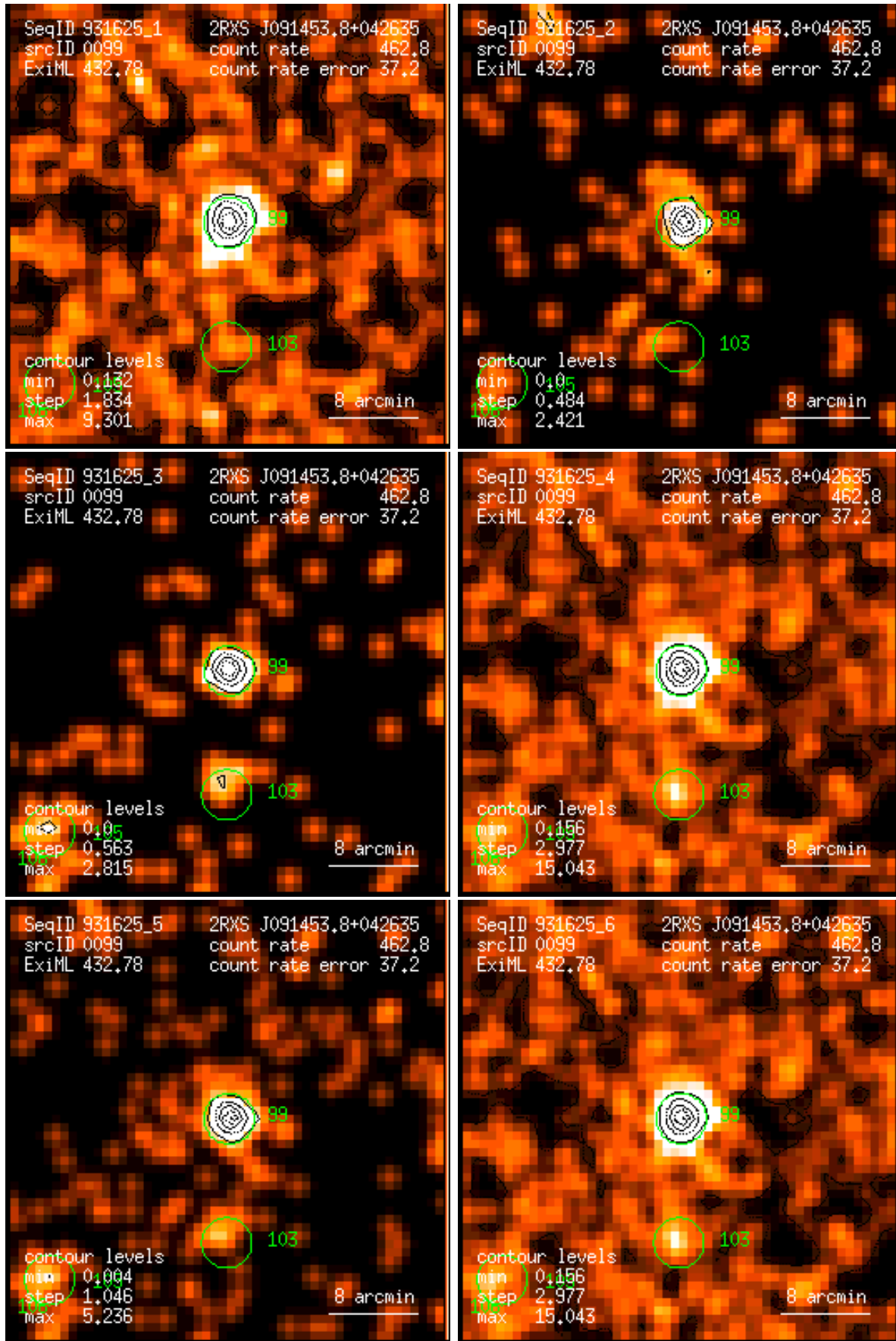
Figure 99: RASS 931625: detection 0099: band rate images, Gaussian filter: (1) PSPC channels 11 – 41, (2) 52 – 90, (3) 91 – 201, (4) 11 – 235, (5) 52 – 201, (6) 11 – 201. Broad band rates in counts/ks. Band rate contour levels in counts/ks/arcmin 2 .
