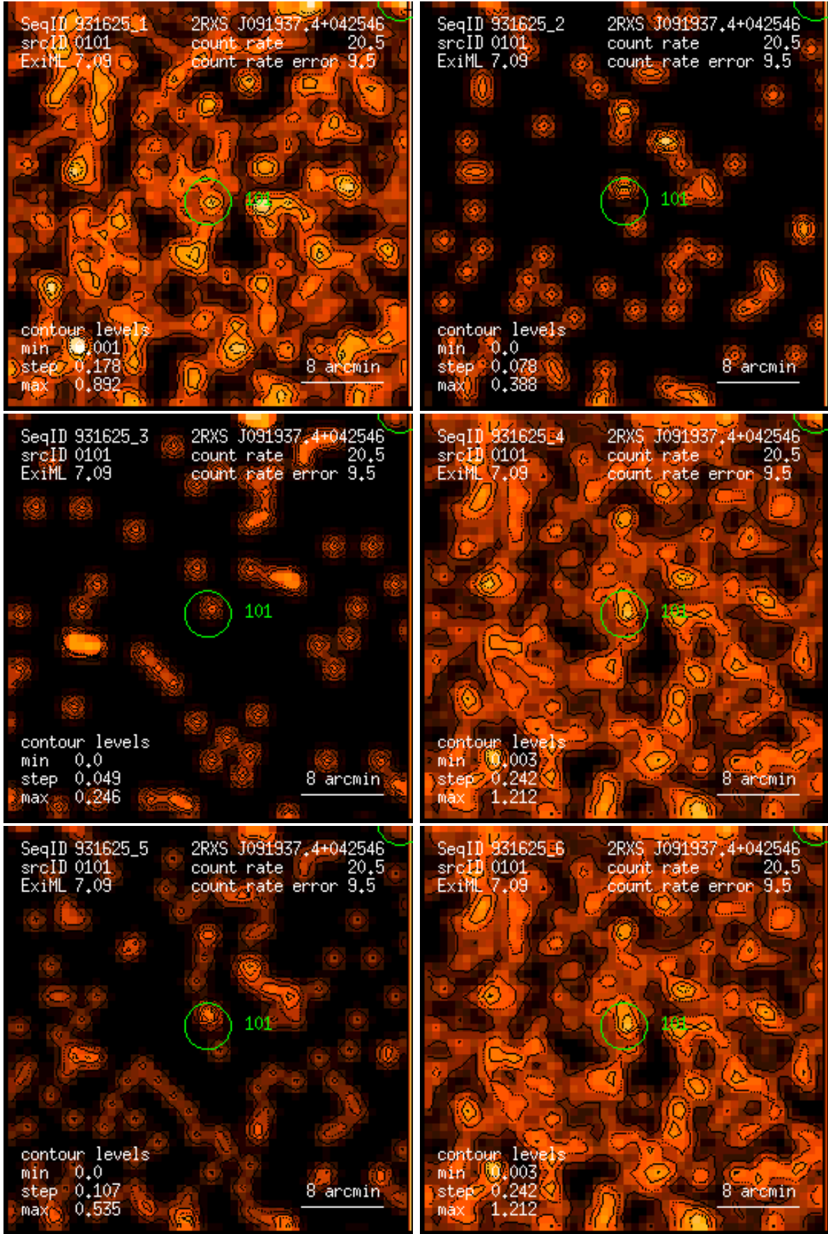
Figure 101: RASS 931625: detection 0101: band rate images, Gaussian filter: (1) PSPC channels 11 – 41, (2) 52 – 90, (3) 91 – 201, (4) 11 – 235, (5) 52 – 201, (6) 11 – 201. Broad band rates in counts/ks. Band rate contour levels in counts/ks/arcmin 2 .
