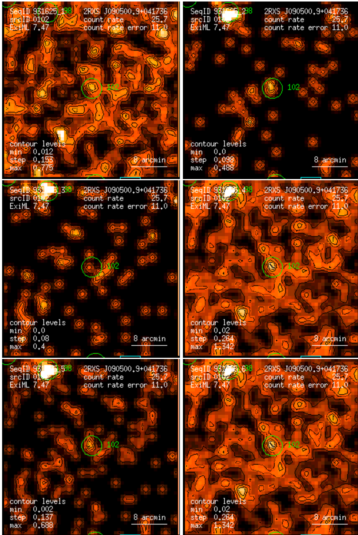
Figure 102: RASS 931625: detection 0102: band rate images, Gaussian filter: (1) PSPC channels 11 – 41, (2) 52 – 90, (3) 91 – 201, (4) 11 – 235, (5) 52 – 201, (6) 11 – 201. Broad band rates in counts/ks. Band rate contour levels in counts/ks/arcmin 2 .
