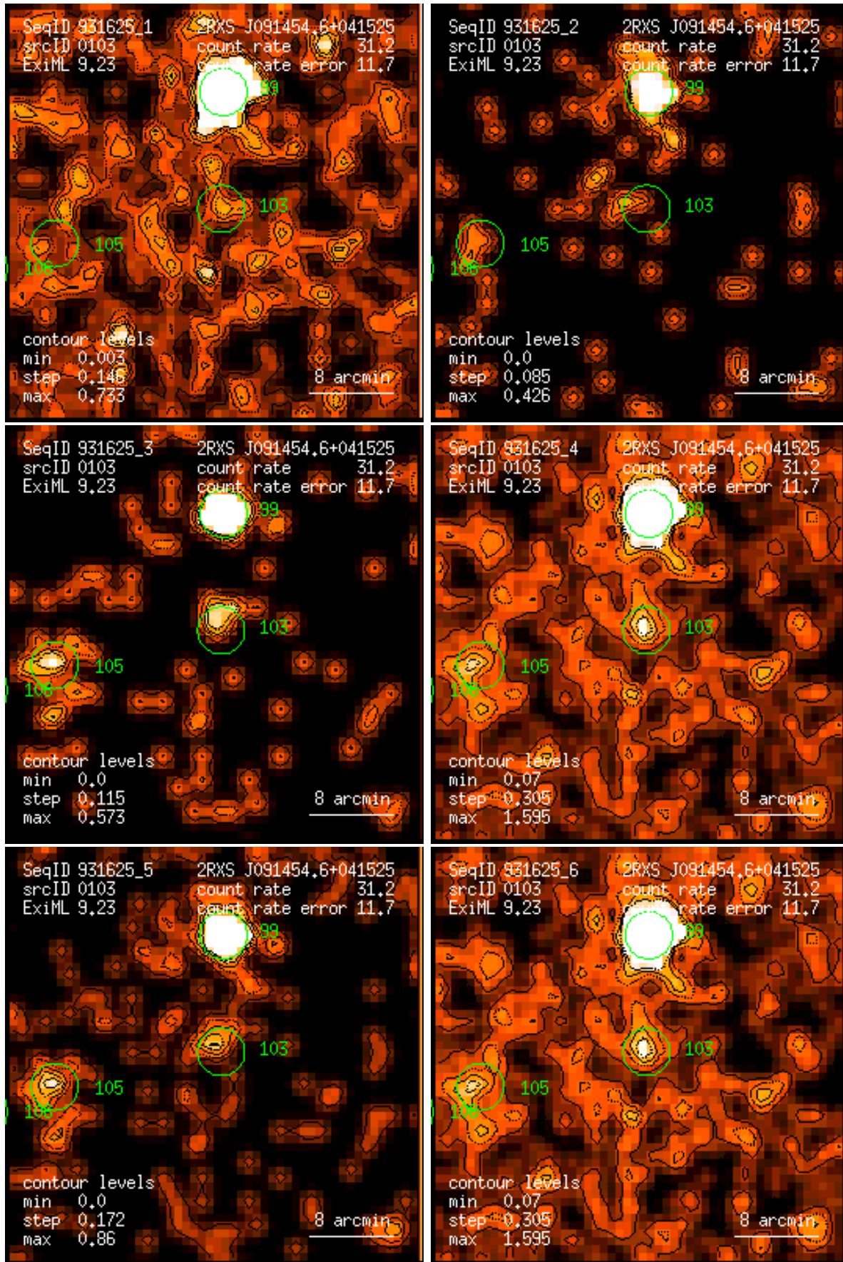
Figure 103: RASS 931625: detection 0103: band rate images, Gaussian filter: (1) PSPC channels 11 – 41, (2) 52 – 90, (3) 91 – 201, (4) 11 – 235, (5) 52 – 201, (6) 11 – 201. Broad band rates in counts/ks. Band rate contour levels in counts/ks/arcmin 2 .
