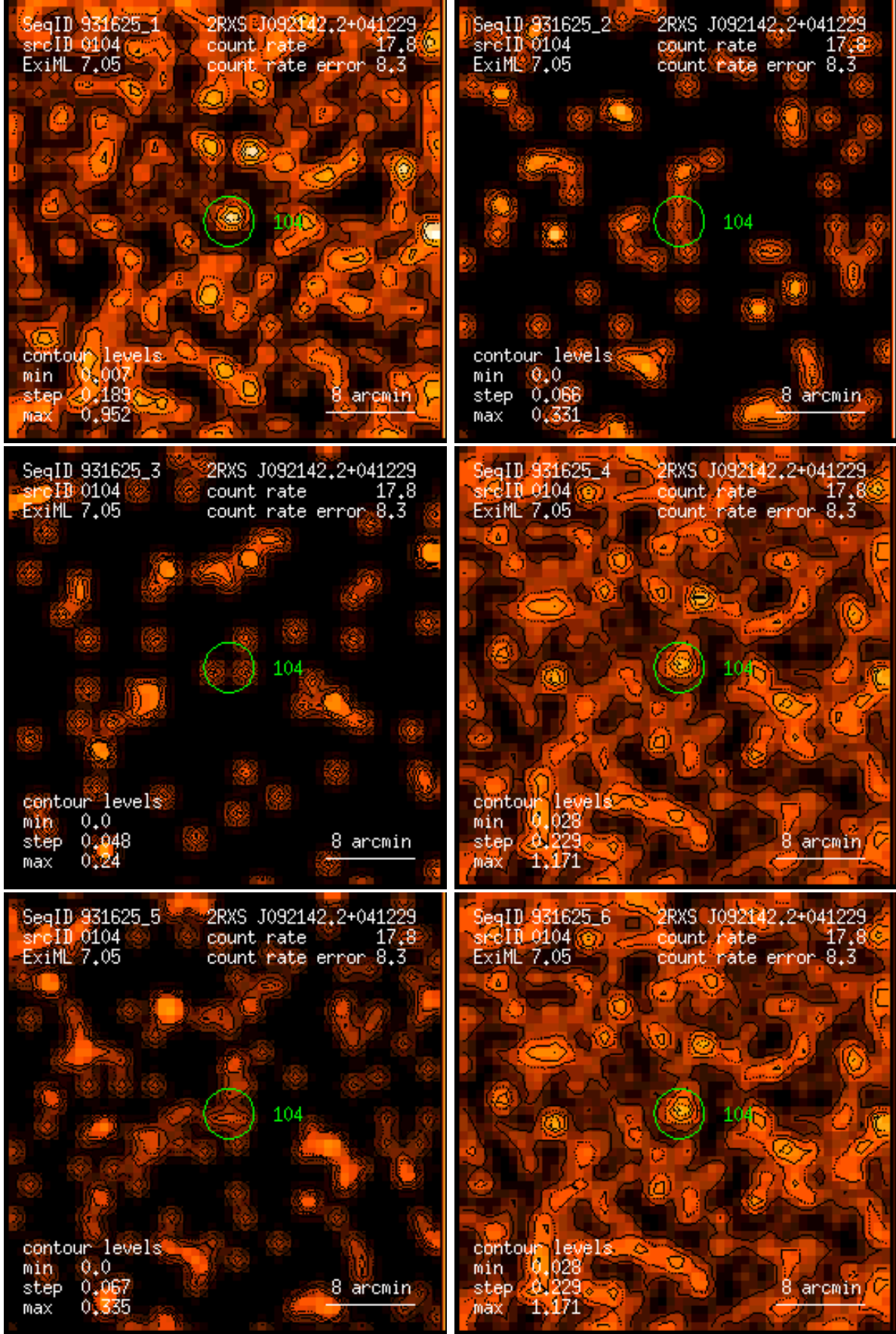
Figure 104: RASS 931625: detection 0104: band rate images, Gaussian filter: (1) PSPC channels 11 – 41, (2) 52 – 90, (3) 91 – 201, (4) 11 – 235, (5) 52 – 201, (6) 11 – 201. Broad band rates in counts/ks. Band rate contour levels in counts/ks/arcmin 2 .
