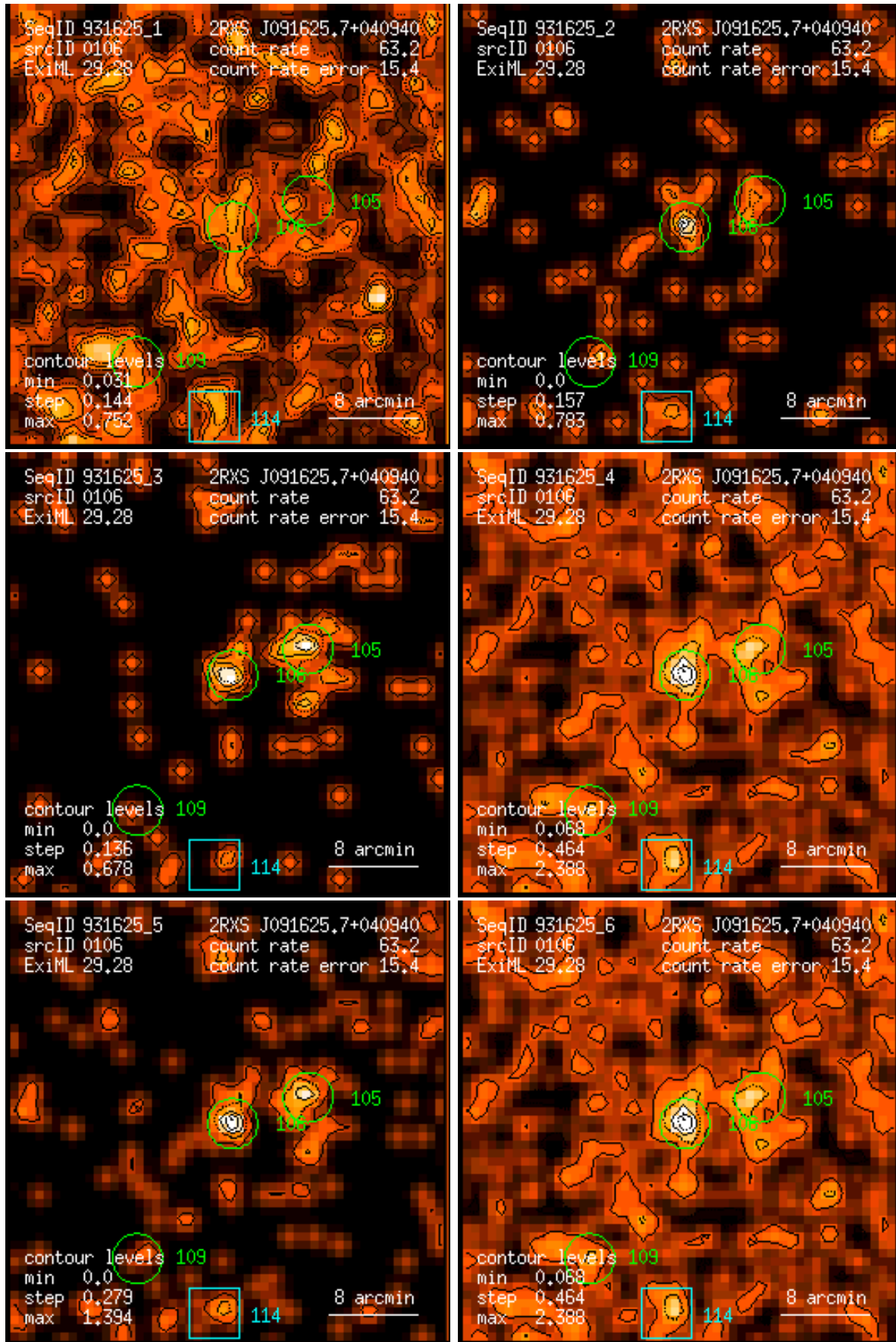
Figure 106: RASS 931625: detection 0106: band rate images, Gaussian filter: (1) PSPC channels 11 – 41, (2) 52 – 90, (3) 91 – 201, (4) 11 – 235, (5) 52 – 201, (6) 11 – 201. Broad band rates in counts/ks. Band rate contour levels in counts/ks/arcmin 2 .
