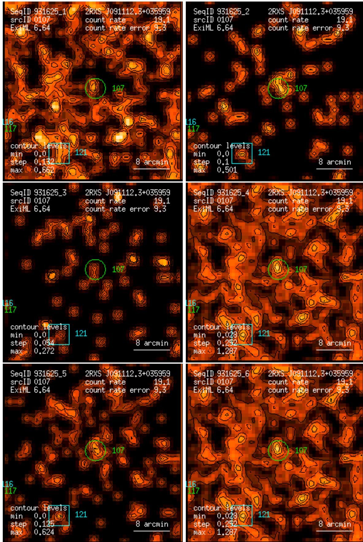
Figure 107: RASS 931625: detection 0107: band rate images, Gaussian filter: (1) PSPC channels 11 – 41, (2) 52 – 90, (3) 91 – 201, (4) 11 – 235, (5) 52 – 201, (6) 11 – 201. Broad band rates in counts/ks. Band rate contour levels in counts/ks/arcmin 2 .
