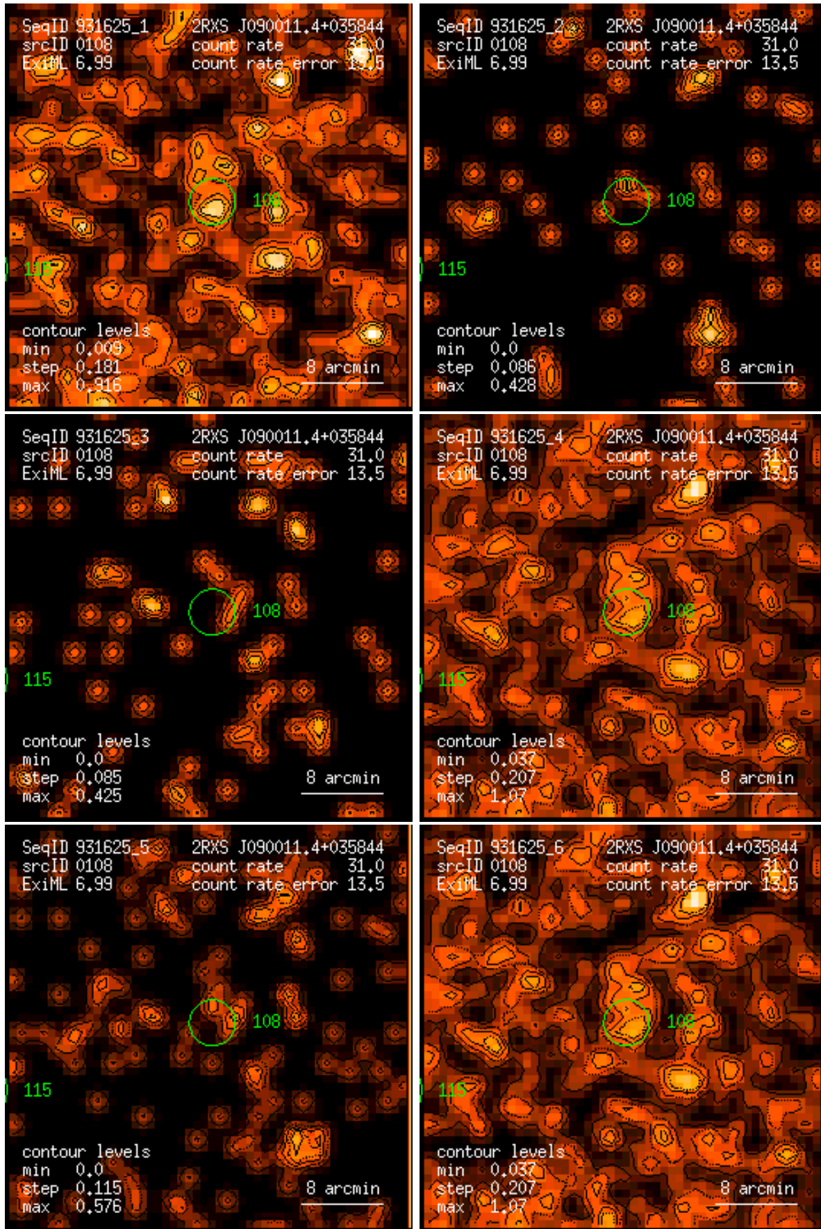
Figure 108: RASS 931625: detection 0108: band rate images, Gaussian filter: (1) PSPC channels 11 – 41, (2) 52 – 90, (3) 91 – 201, (4) 11 – 235, (5) 52 – 201, (6) 11 – 201. Broad band rates in counts/ks. Band rate contour levels in counts/ks/arcmin 2 .
