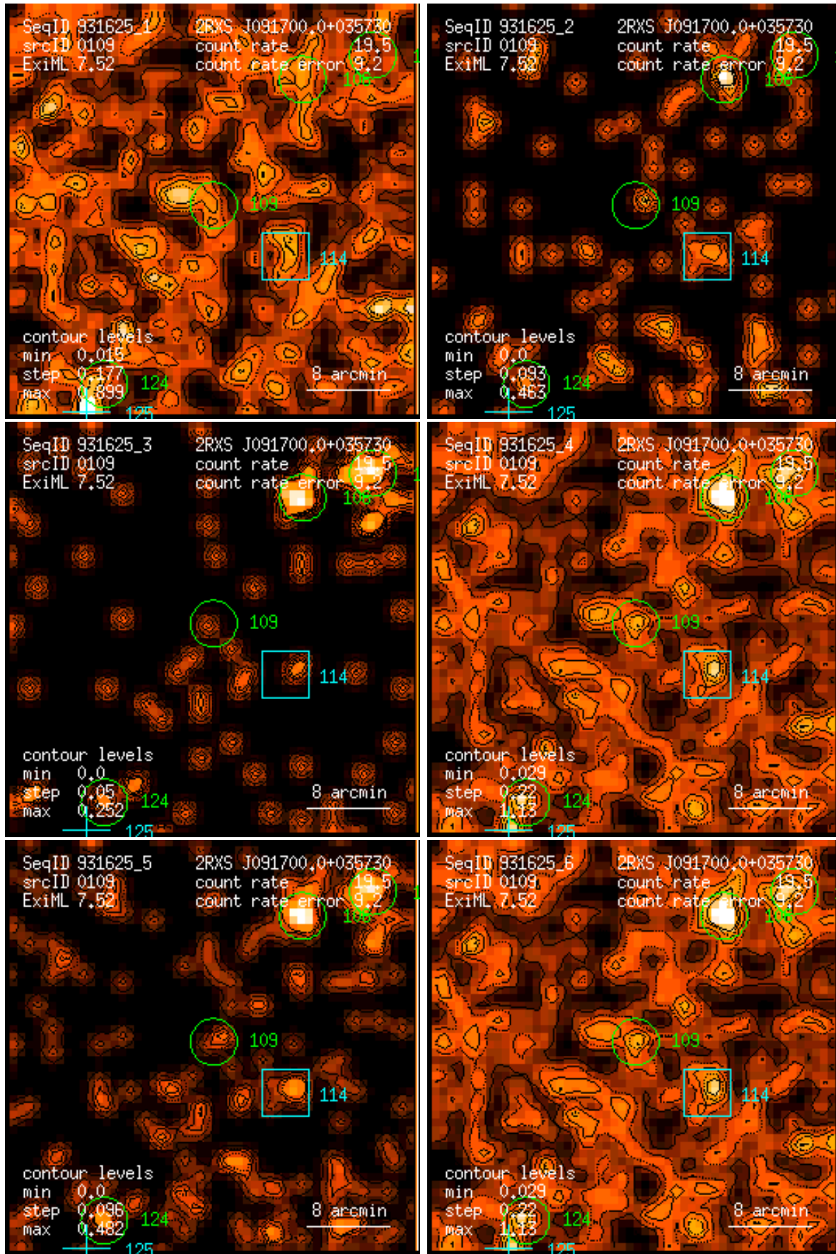
Figure 109: RASS 931625: detection 0109: band rate images, Gaussian filter: (1) PSPC channels 11 – 41, (2) 52 – 90, (3) 91 – 201, (4) 11 – 235, (5) 52 – 201, (6) 11 – 201. Broad band rates in counts/ks. Band rate contour levels in counts/ks/arcmin 2 .
