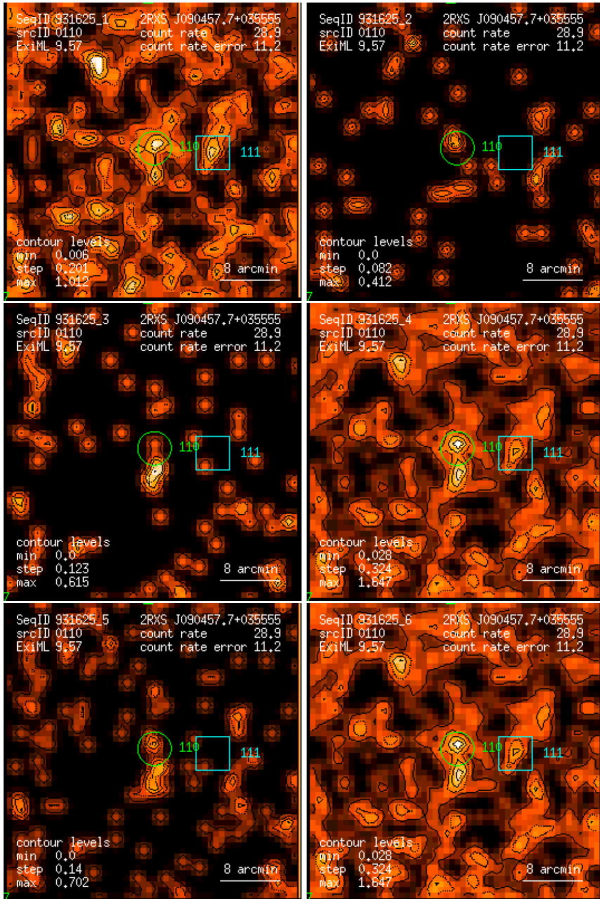
Figure 110: RASS 931625: detection 0110: band rate images, Gaussian filter: (1) PSPC channels 11 – 41, (2) 52 – 90, (3) 91 – 201, (4) 11 – 235, (5) 52 – 201, (6) 11 – 201. Broad band rates in counts/ks. Band rate contour levels in counts/ks/arcmin 2 .
