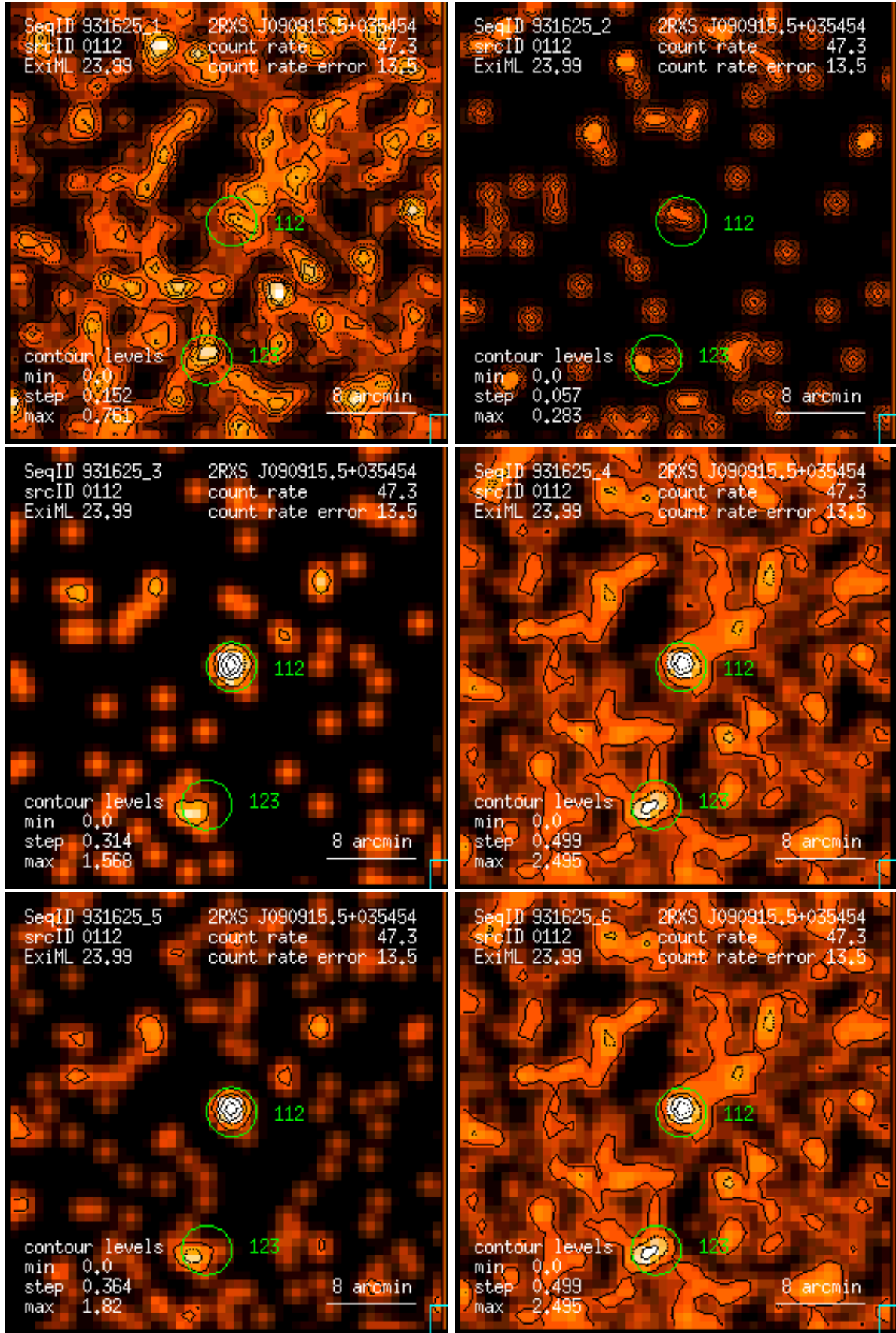
Figure 112: RASS 931625: detection 0112: band rate images, Gaussian filter: (1) PSPC channels 11 – 41, (2) 52 – 90, (3) 91 – 201, (4) 11 – 235, (5) 52 – 201, (6) 11 – 201. Broad band rates in counts/ks. Band rate contour levels in counts/ks/arcmin 2 .
