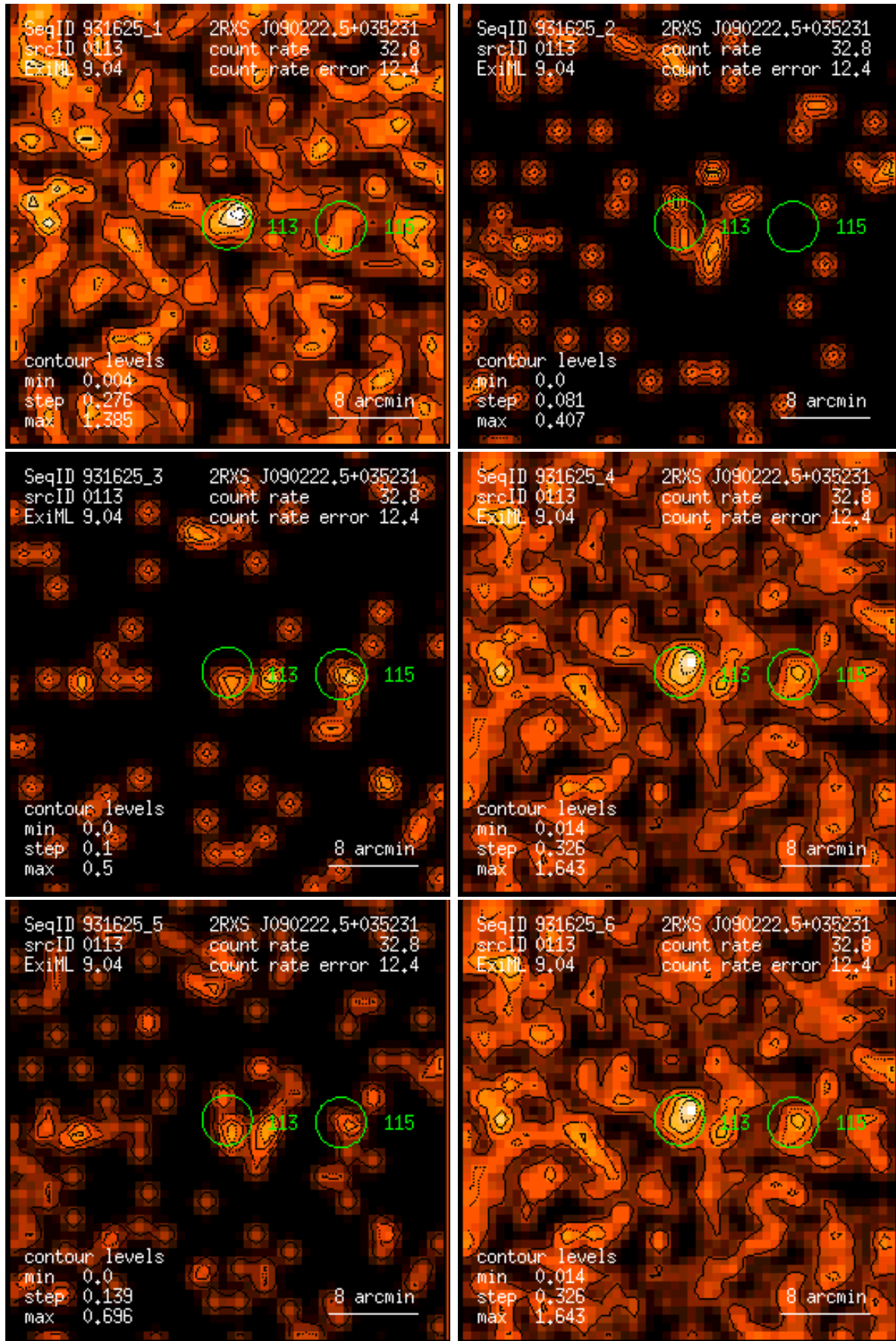
Figure 113: RASS 931625: detection 0113: band rate images, Gaussian filter: (1) PSPC channels 11 – 41, (2) 52 – 90, (3) 91 – 201, (4) 11 – 235, (5) 52 – 201, (6) 11 – 201. Broad band rates in counts/ks. Band rate contour levels in counts/ks/arcmin 2 .
