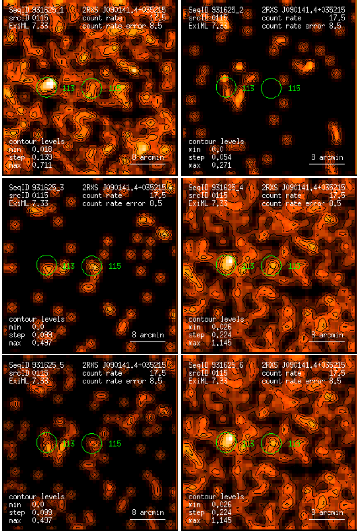
Figure 115: RASS 931625: detection 0115: band rate images, Gaussian filter: (1) PSPC channels 11 – 41, (2) 52 – 90, (3) 91 – 201, (4) 11 – 235, (5) 52 – 201, (6) 11 – 201. Broad band rates in counts/ks. Band rate contour levels in counts/ks/arcmin 2 .
