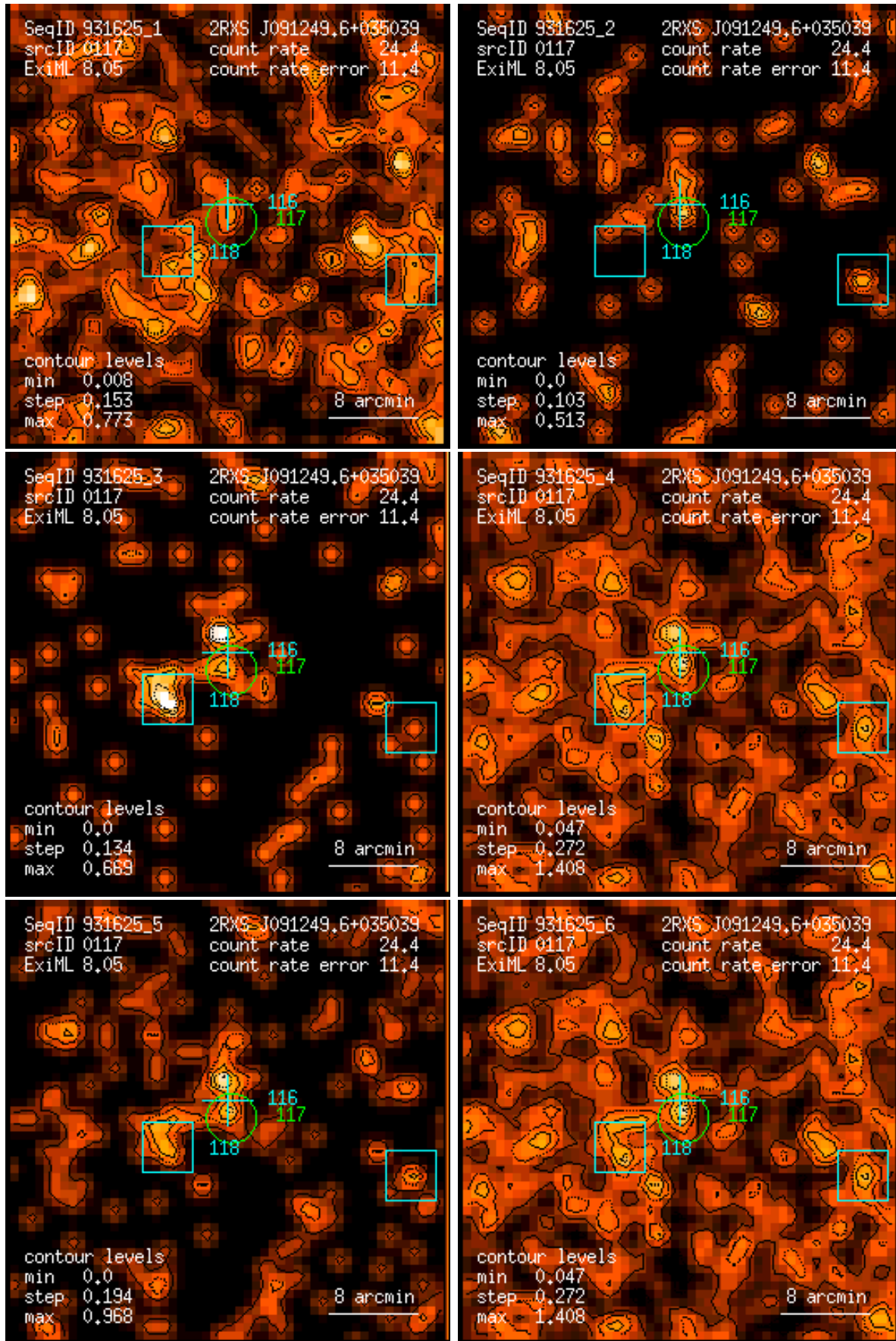
Figure 117: RASS 931625: detection 0117: band rate images, Gaussian filter: (1) PSPC channels 11 – 41, (2) 52 – 90, (3) 91 – 201, (4) 11 – 235, (5) 52 – 201, (6) 11 – 201. Broad band rates in counts/ks. Band rate contour levels in counts/ks/arcmin 2 .
