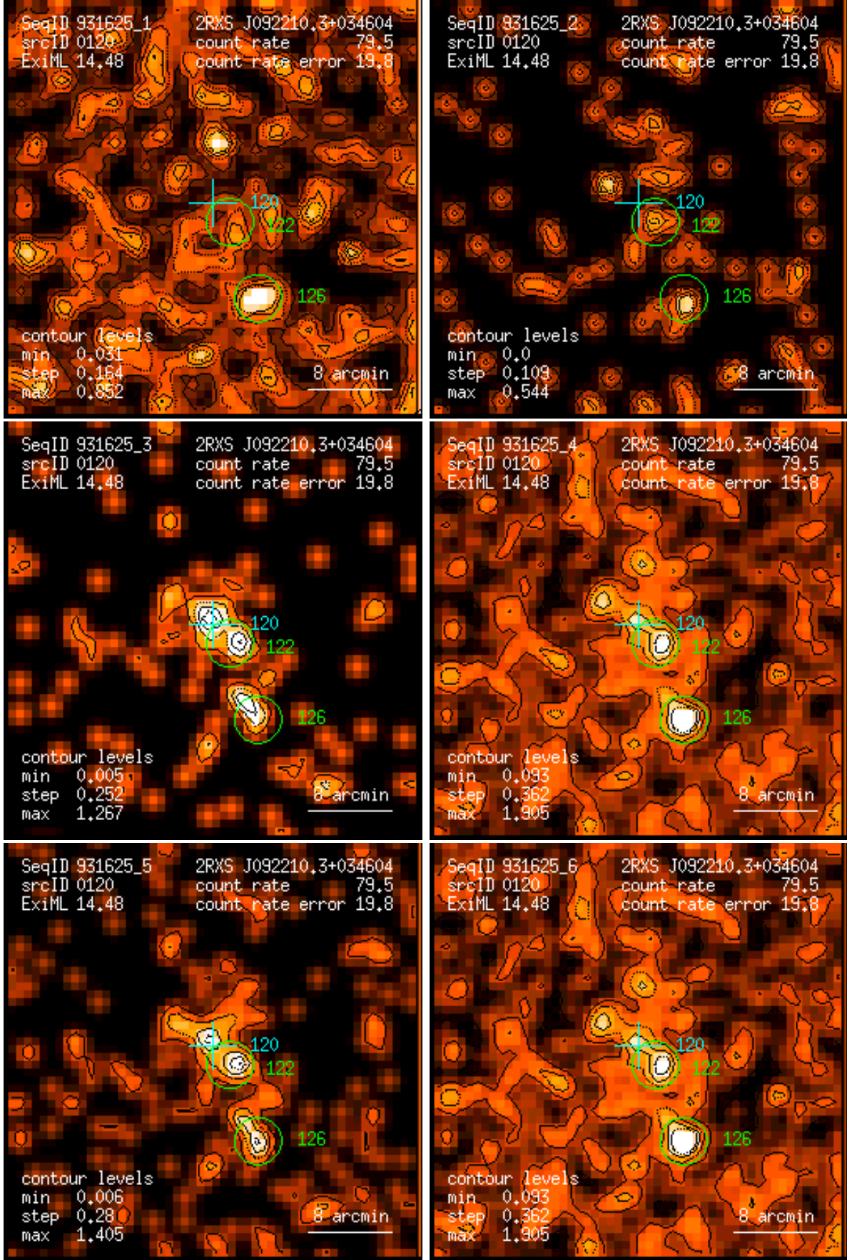
Figure 120: RASS 931625: detection 0120: band rate images, Gaussian filter: (1) PSPC channels 11 – 41, (2) 52 – 90, (3) 91 – 201, (4) 11 – 235, (5) 52 – 201, (6) 11 – 201. Broad band rates in counts/ks. Band rate contour levels in counts/ks/arcmin 2 .
