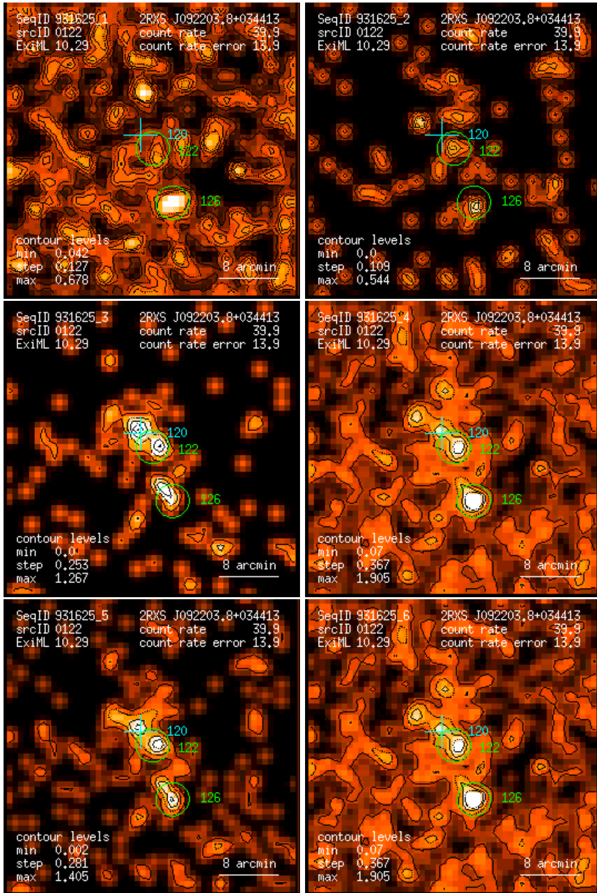
Figure 122: RASS 931625: detection 0122: band rate images, Gaussian filter: (1) PSPC channels 11 – 41, (2) 52 – 90, (3) 91 – 201, (4) 11 – 235, (5) 52 – 201, (6) 11 – 201. Broad band rates in counts/ks. Band rate contour levels in counts/ks/arcmin 2 .
