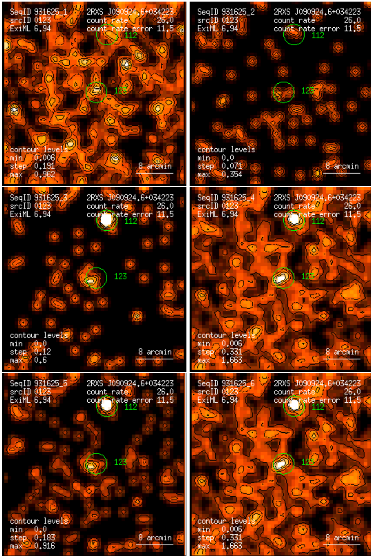
Figure 123: RASS 931625: detection 0123: band rate images, Gaussian filter: (1) PSPC channels 11 – 41, (2) 52 – 90, (3) 91 – 201, (4) 11 – 235, (5) 52 – 201, (6) 11 – 201. Broad band rates in counts/ks. Band rate contour levels in counts/ks/arcmin 2 .
