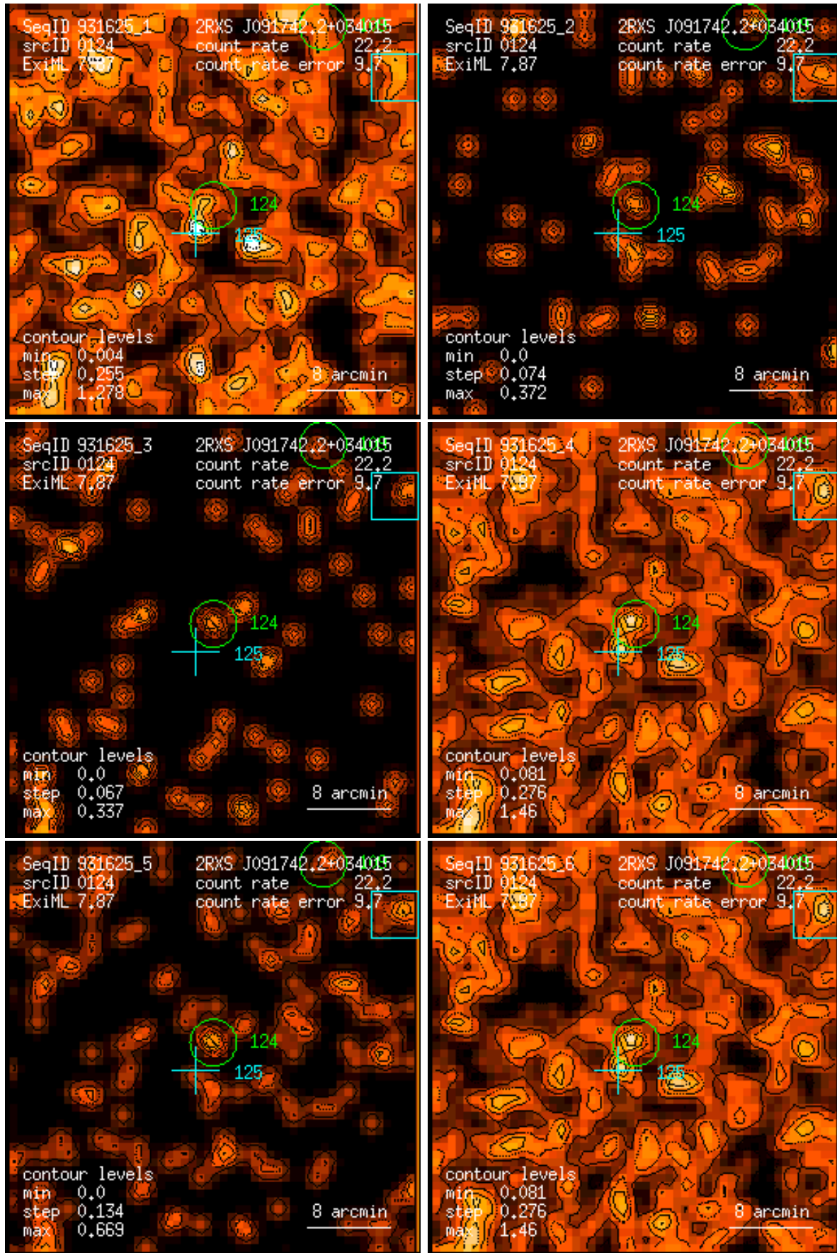
Figure 124: RASS 931625: detection 0124: band rate images, Gaussian filter: (1) PSPC channels 11 – 41, (2) 52 – 90, (3) 91 – 201, (4) 11 – 235, (5) 52 – 201, (6) 11 – 201. Broad band rates in counts/ks. Band rate contour levels in counts/ks/arcmin 2 .
