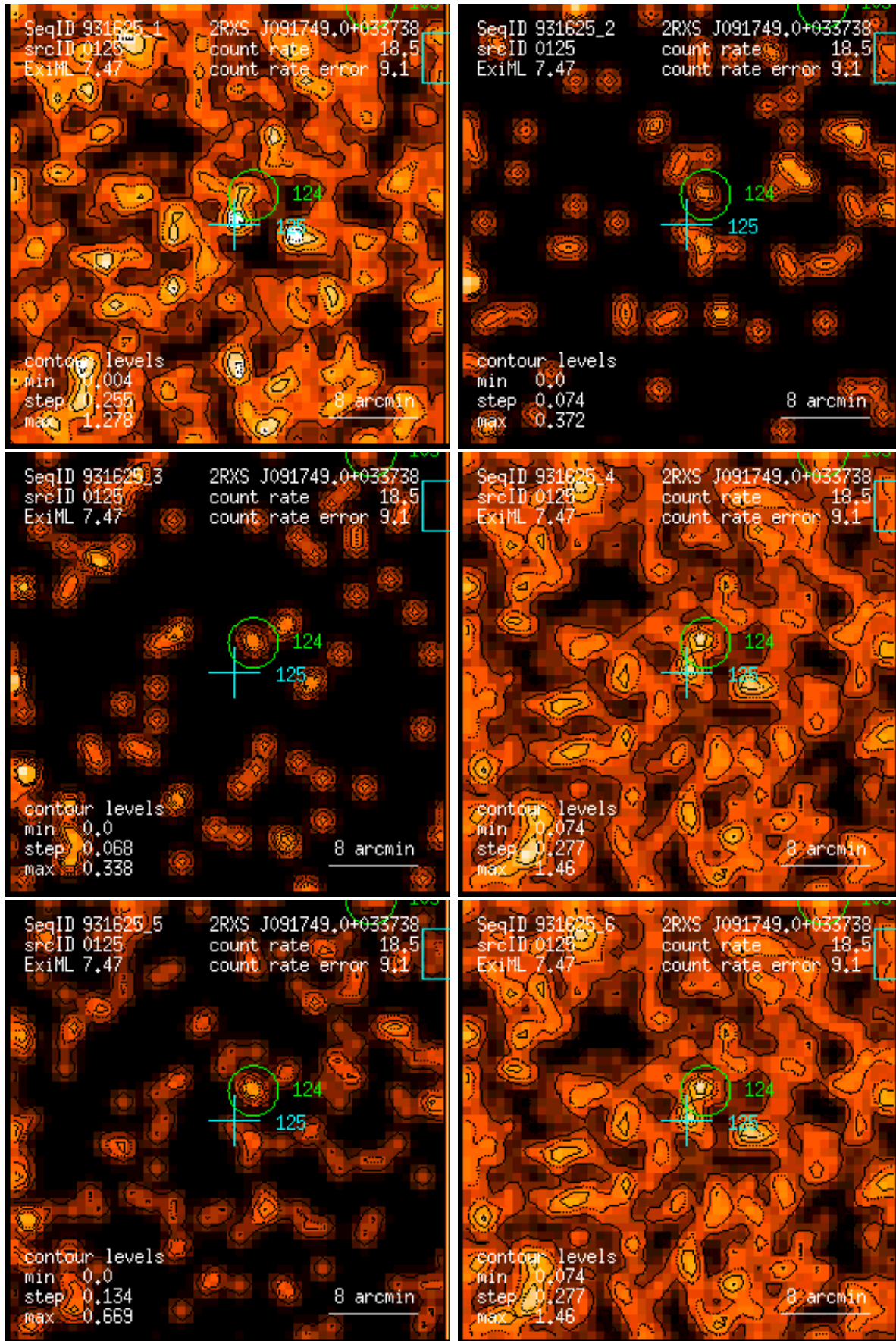
Figure 125: RASS 931625: detection 0125: band rate images, Gaussian filter: (1) PSPC channels 11 – 41, (2) 52 – 90, (3) 91 – 201, (4) 11 – 235, (5) 52 – 201, (6) 11 – 201. Broad band rates in counts/ks. Band rate contour levels in counts/ks/arcmin 2 .
