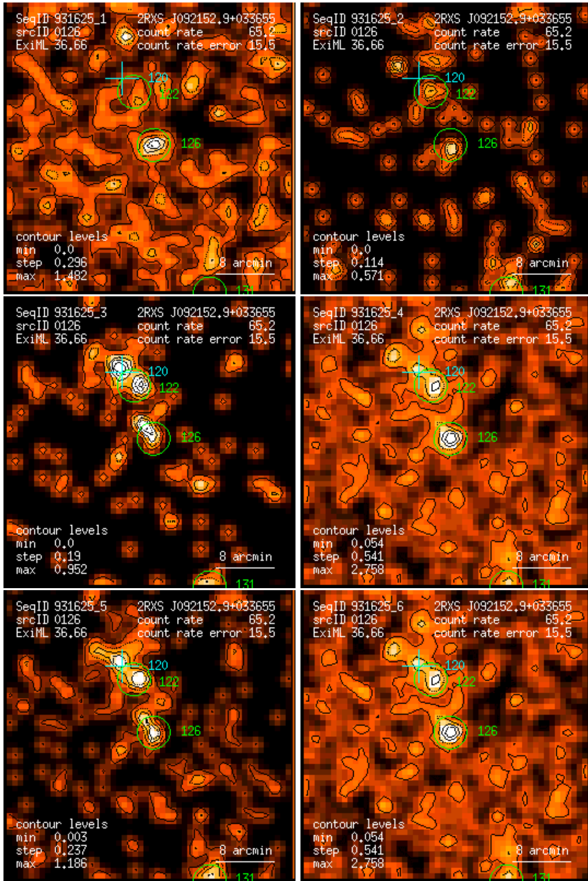
Figure 126: RASS 931625: detection 0126: band rate images, Gaussian filter: (1) PSPC channels 11 – 41, (2) 52 – 90, (3) 91 – 201, (4) 11 – 235, (5) 52 – 201, (6) 11 – 201. Broad band rates in counts/ks. Band rate contour levels in counts/ks/arcmin 2 .
