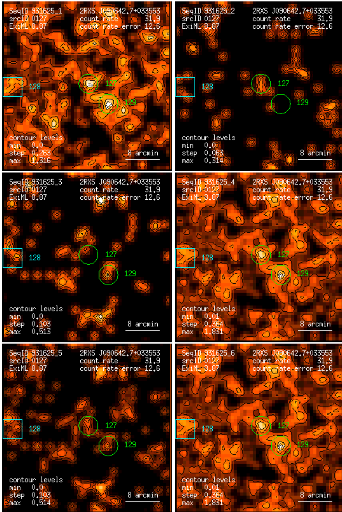
Figure 127: RASS 931625: detection 0127: band rate images, Gaussian filter: (1) PSPC channels 11 – 41, (2) 52 – 90, (3) 91 – 201, (4) 11 – 235, (5) 52 – 201, (6) 11 – 201. Broad band rates in counts/ks. Band rate contour levels in counts/ks/arcmin 2 .
