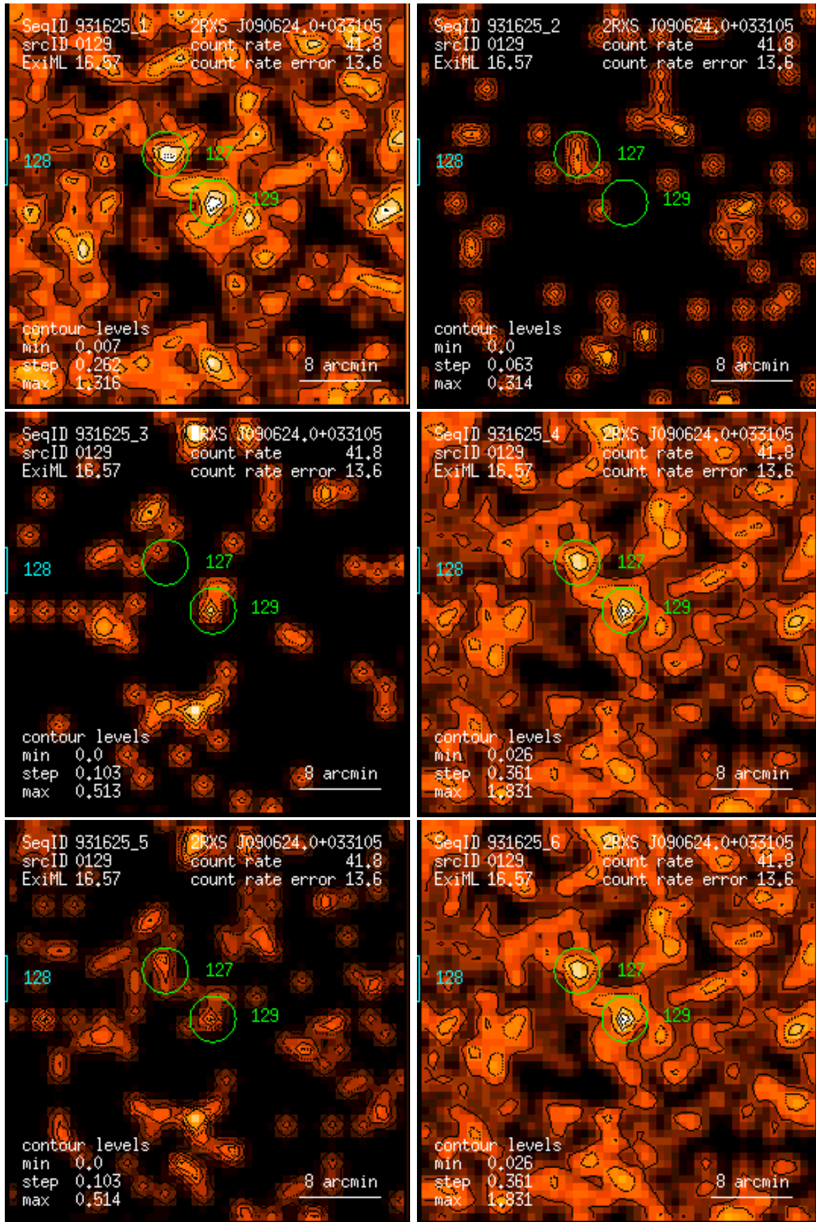
Figure 129: RASS 931625: detection 0129: band rate images, Gaussian filter: (1) PSPC channels 11 – 41, (2) 52 – 90, (3) 91 – 201, (4) 11 – 235, (5) 52 – 201, (6) 11 – 201. Broad band rates in counts/ks. Band rate contour levels in counts/ks/arcmin 2 .
