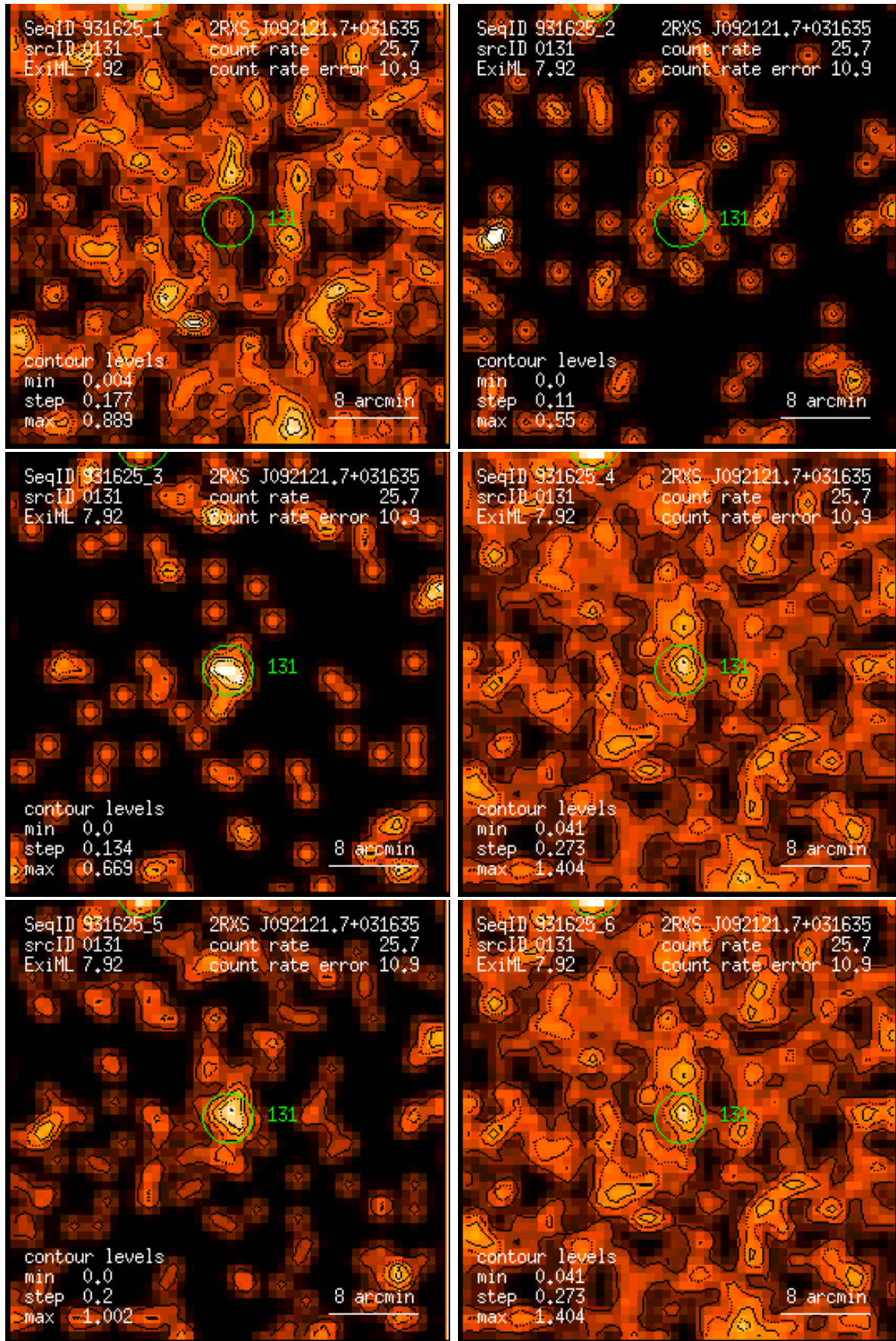
Figure 131: RASS 931625: detection 0131: band rate images, Gaussian filter: (1) PSPC channels 11 – 41, (2) 52 – 90, (3) 91 – 201, (4) 11 – 235, (5) 52 – 201, (6) 11 – 201. Broad band rates in counts/ks. Band rate contour levels in counts/ks/arcmin 2 .
