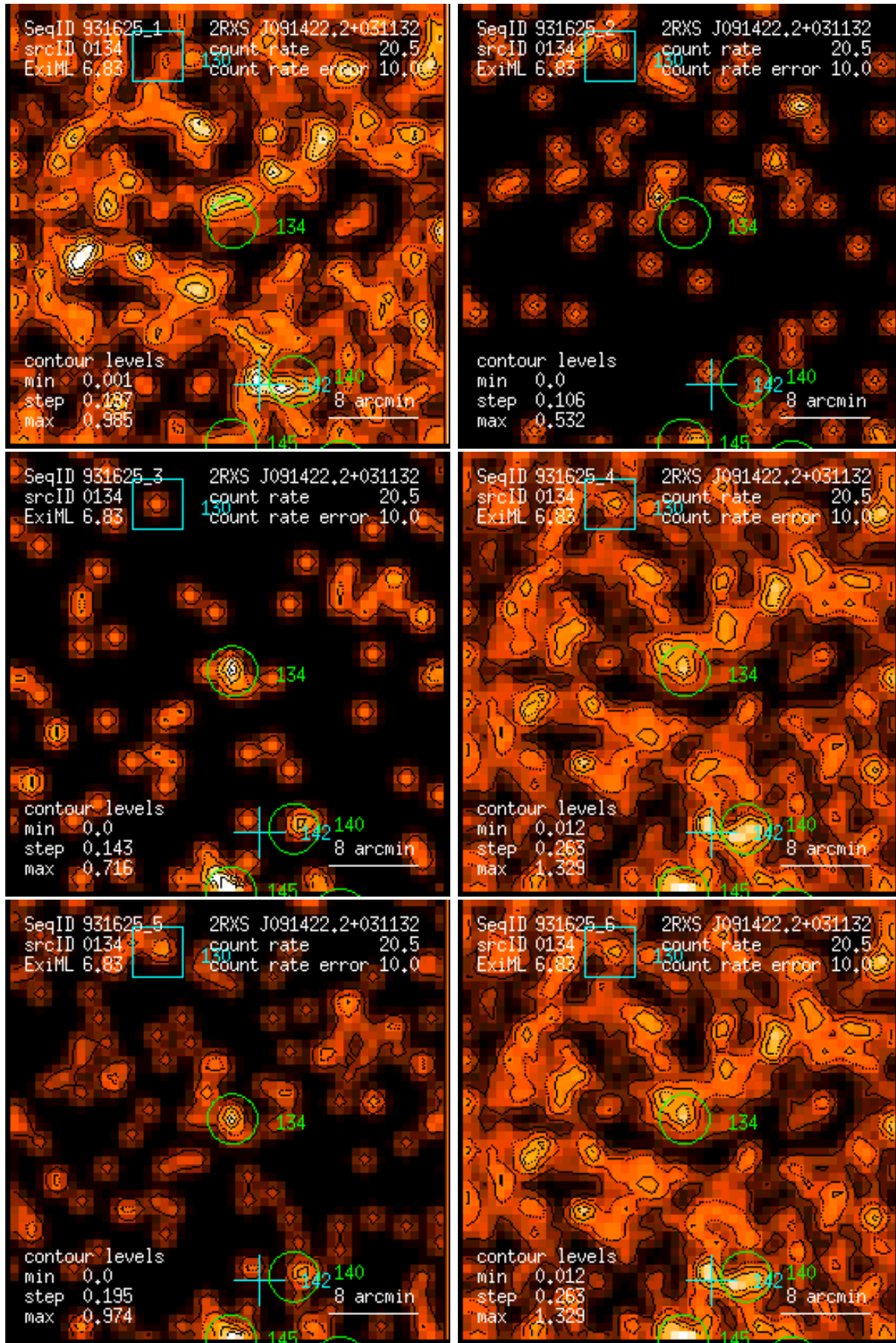
Figure 134: RASS 931625: detection 0134: band rate images, Gaussian filter: (1) PSPC channels 11 – 41, (2) 52 – 90, (3) 91 – 201, (4) 11 – 235, (5) 52 – 201, (6) 11 – 201. Broad band rates in counts/ks. Band rate contour levels in counts/ks/arcmin 2 .
