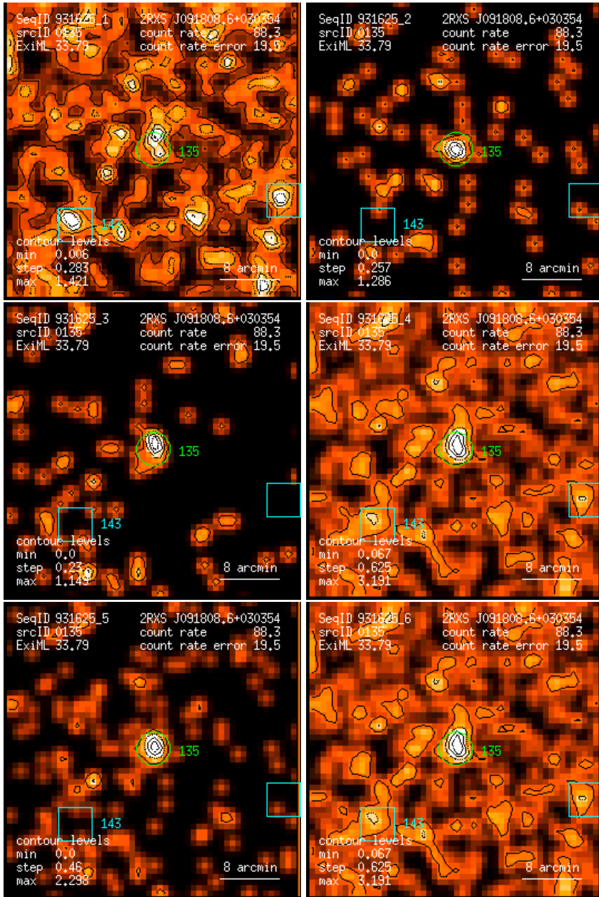
Figure 135: RASS 931625: detection 0135: band rate images, Gaussian filter: (1) PSPC channels 11 – 41, (2) 52 – 90, (3) 91 – 201, (4) 11 – 235, (5) 52 – 201, (6) 11 – 201. Broad band rates in counts/ks. Band rate contour levels in counts/ks/arcmin 2 .
