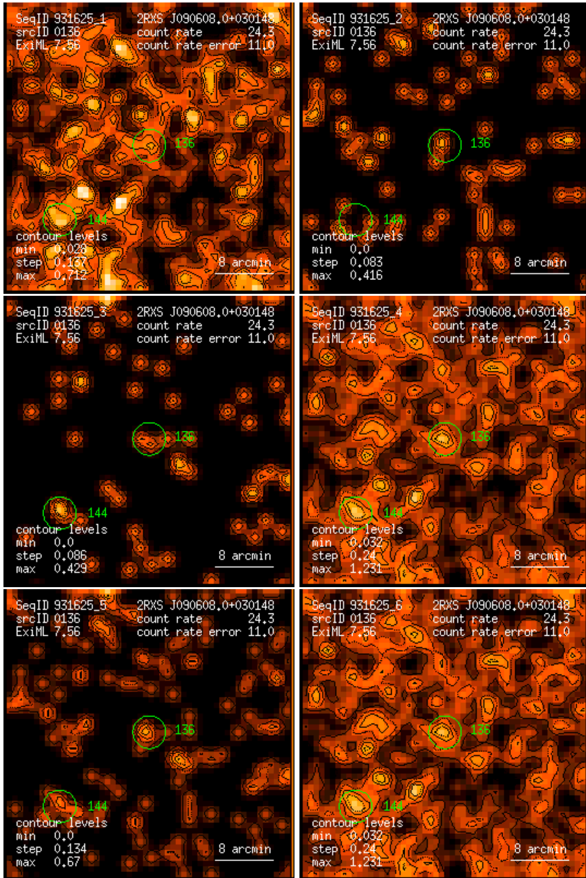
Figure 136: RASS 931625: detection 0136: band rate images, Gaussian filter: (1) PSPC channels 11 – 41, (2) 52 – 90, (3) 91 – 201, (4) 11 – 235, (5) 52 – 201, (6) 11 – 201. Broad band rates in counts/ks. Band rate contour levels in counts/ks/arcmin 2 .
