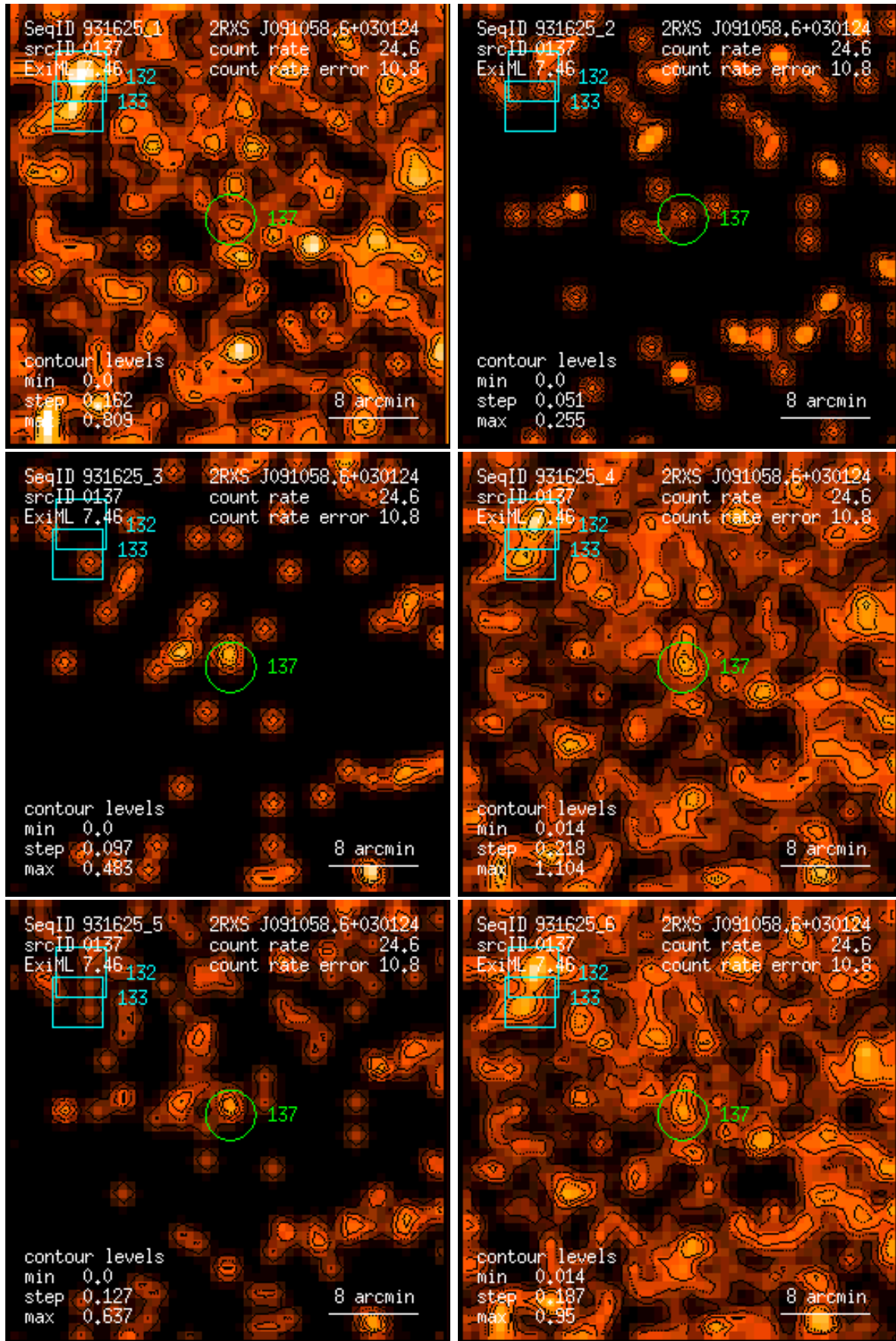
Figure 137: RASS 931625: detection 0137: band rate images, Gaussian filter: (1) PSPC channels 11 – 41, (2) 52 – 90, (3) 91 – 201, (4) 11 – 235, (5) 52 – 201, (6) 11 – 201. Broad band rates in counts/ks. Band rate contour levels in counts/ks/arcmin 2 .
