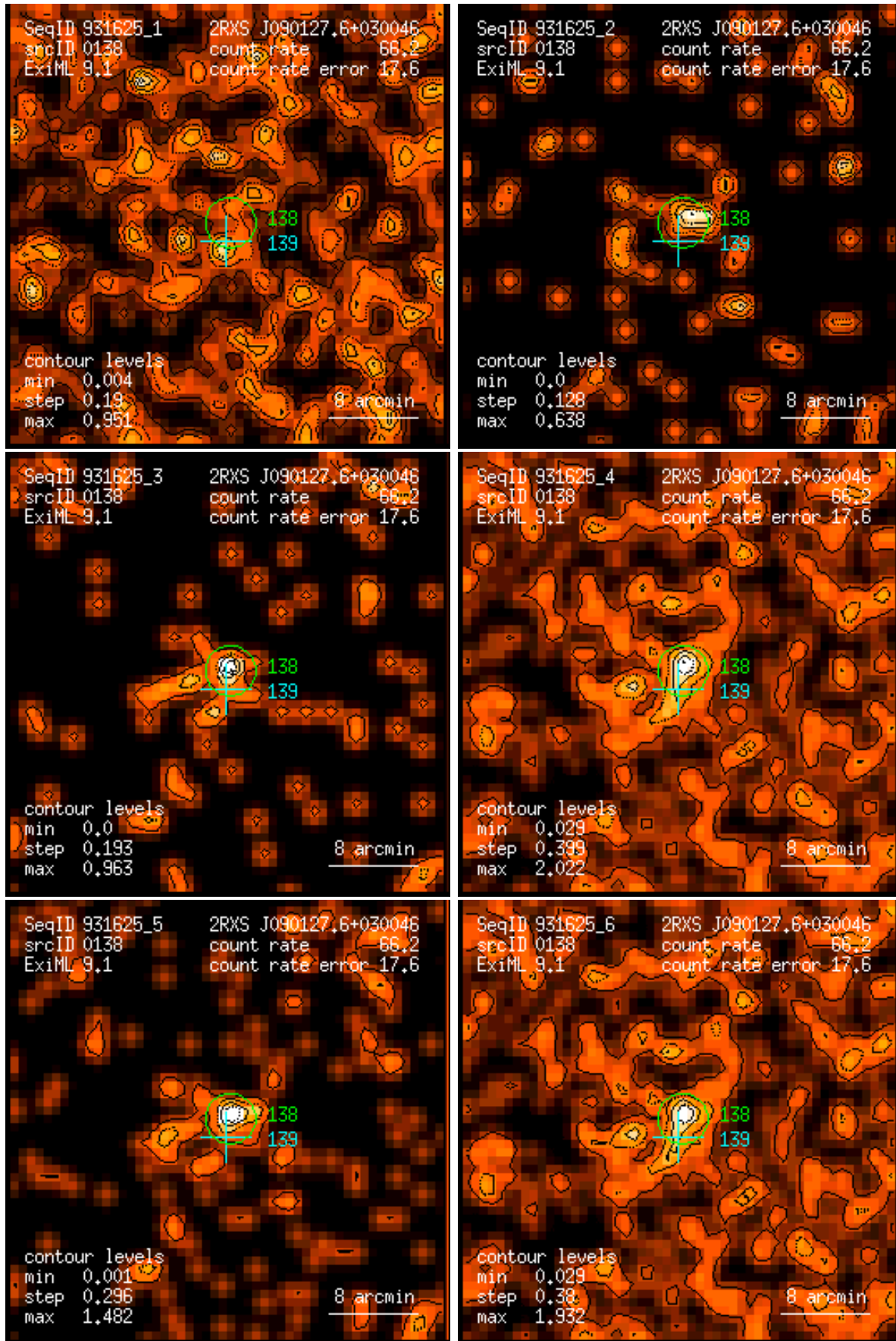
Figure 138: RASS 931625: detection 0138: band rate images, Gaussian filter: (1) PSPC channels 11 – 41, (2) 52 – 90, (3) 91 – 201, (4) 11 – 235, (5) 52 – 201, (6) 11 – 201. Broad band rates in counts/ks. Band rate contour levels in counts/ks/arcmin 2 .
