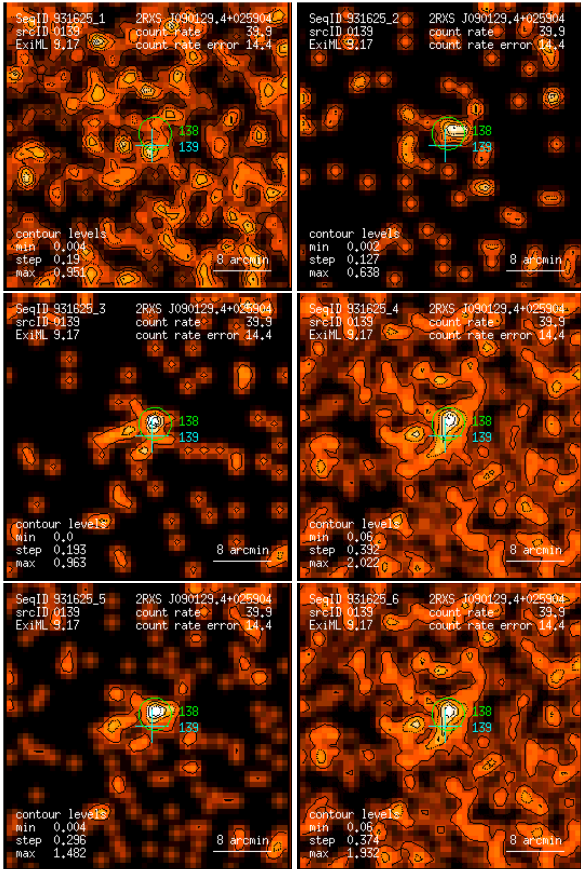
Figure 139: RASS 931625: detection 0139: band rate images, Gaussian filter: (1) PSPC channels 11 – 41, (2) 52 – 90, (3) 91 – 201, (4) 11 – 235, (5) 52 – 201, (6) 11 – 201. Broad band rates in counts/ks. Band rate contour levels in counts/ks/arcmin 2 .
