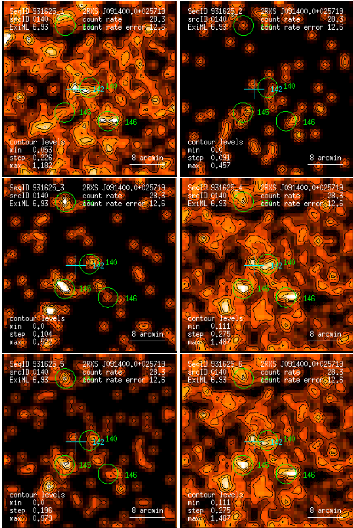
Figure 140: RASS 931625: detection 0140: band rate images, Gaussian filter: (1) PSPC channels 11 – 41, (2) 52 – 90, (3) 91 – 201, (4) 11 – 235, (5) 52 – 201, (6) 11 – 201. Broad band rates in counts/ks. Band rate contour levels in counts/ks/arcmin 2 .
