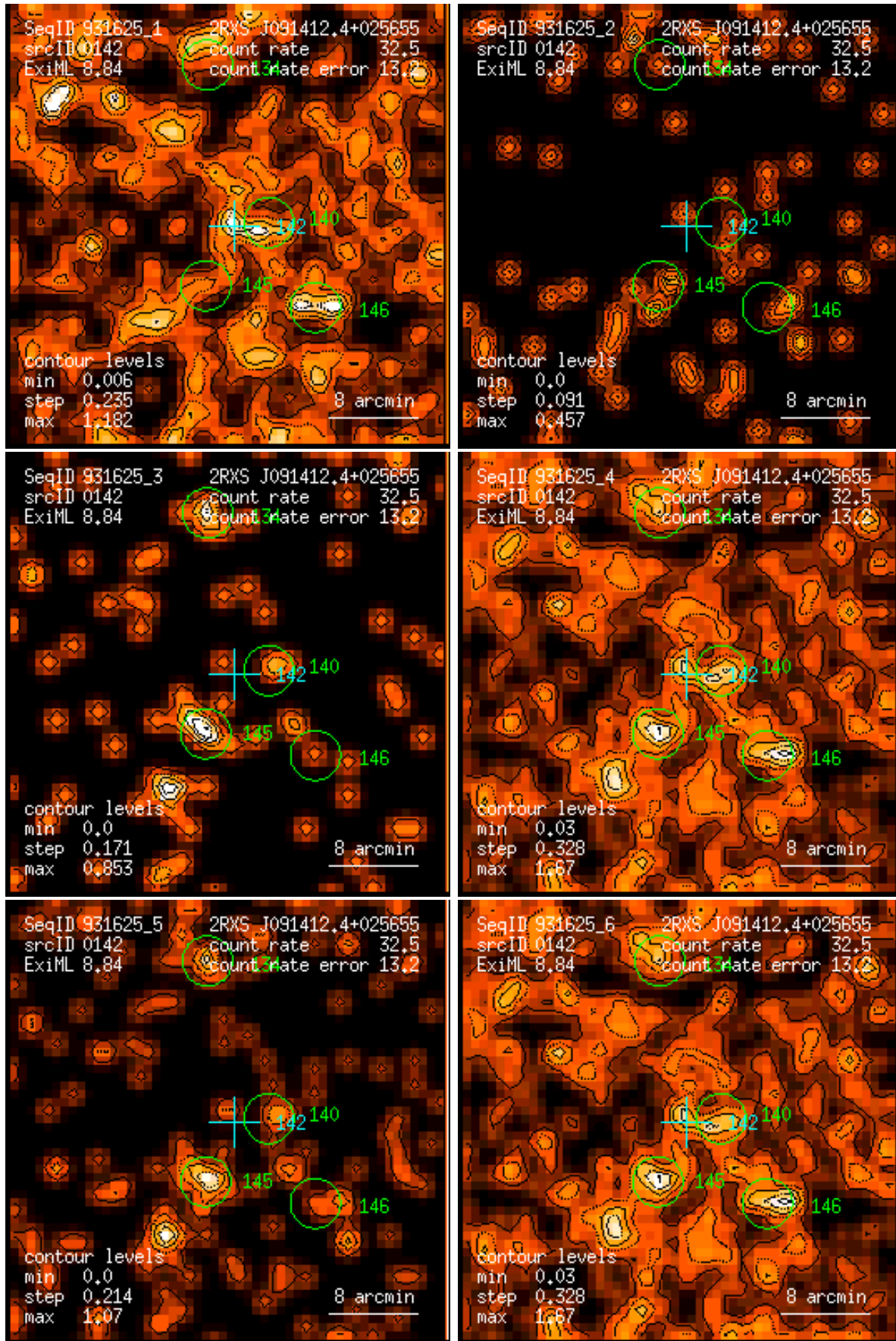
Figure 142: RASS 931625: detection 0142: band rate images, Gaussian filter: (1) PSPC channels 11 – 41, (2) 52 – 90, (3) 91 – 201, (4) 11 – 235, (5) 52 – 201, (6) 11 – 201. Broad band rates in counts/ks. Band rate contour levels in counts/ks/arcmin 2 .
