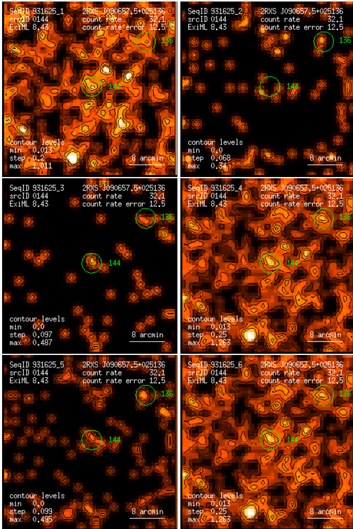
Figure 144: RASS 931625: detection 0144: band rate images, Gaussian filter: (1) PSPC channels 11 – 41, (2) 52 – 90, (3) 91 – 201, (4) 11 – 235, (5) 52 – 201, (6) 11 – 201. Broad band rates in counts/ks. Band rate contour levels in counts/ks/arcmin 2 .
