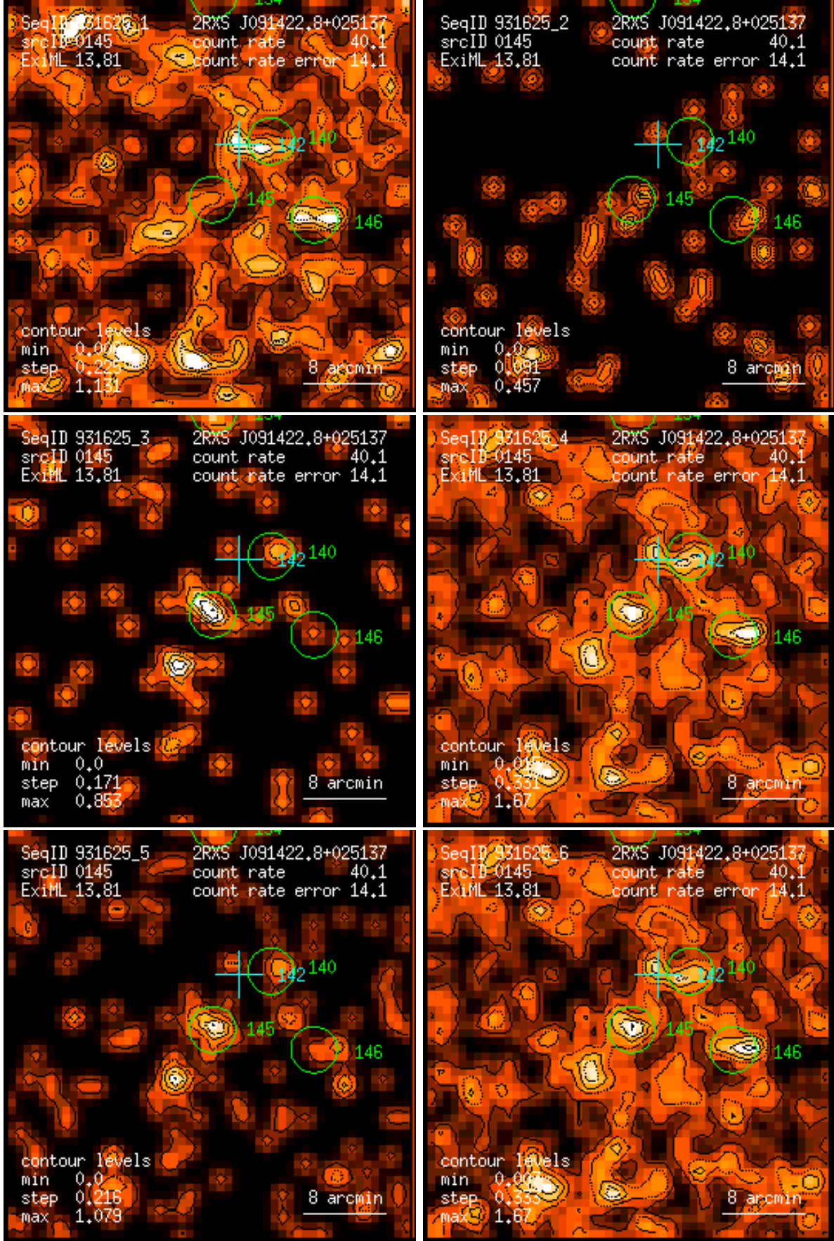
Figure 145: RASS 931625: detection 0145: band rate images, Gaussian filter: (1) PSPC channels 11 – 41, (2) 52 – 90, (3) 91 – 201, (4) 11 – 235, (5) 52 – 201, (6) 11 – 201. Broad band rates in counts/ks. Band rate contour levels in counts/ks/arcmin 2 .
