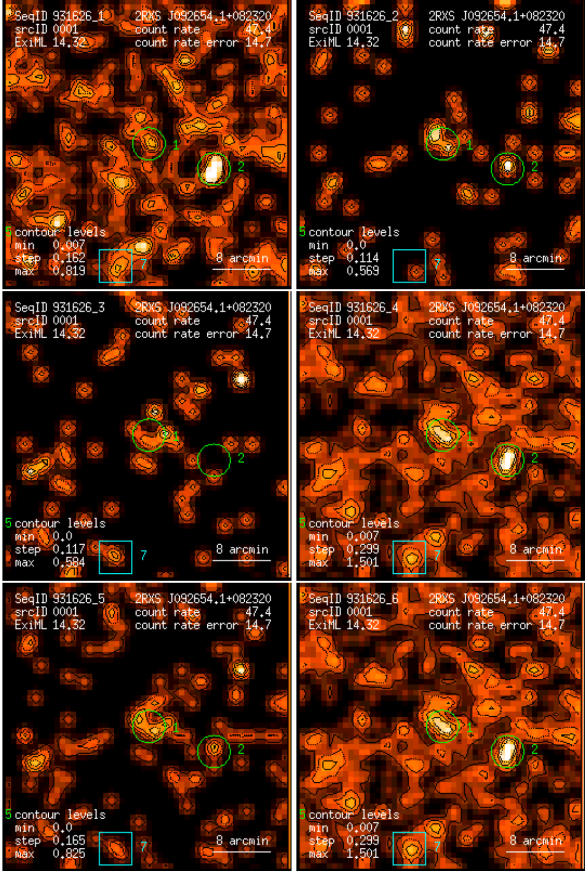
Figure 1: RASS 931626: detection 0001: band rate images, Gaussian filter: (1) PSPC channels 11 – 41, (2) 52 – 90, (3) 91 – 201, (4) 11 – 235, (5) 52 – 201, (6) 11 – 201. Broad band rates in counts/ks. Band rate contour levels in counts/ks/arcmin 2 .
