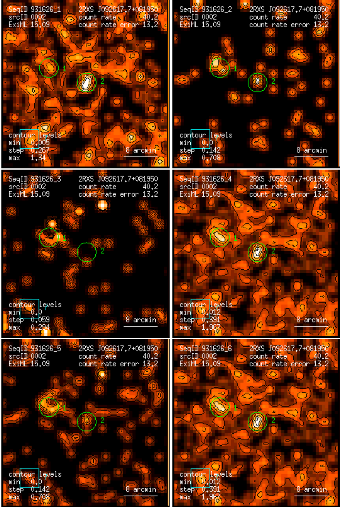
Figure 2: RASS 931626: detection 0002: band rate images, Gaussian filter: (1) PSPC channels 11 – 41, (2) 52 – 90, (3) 91 – 201, (4) 11 – 235, (5) 52 – 201, (6) 11 – 201. Broad band rates in counts/ks. Band rate contour levels in counts/ks/arcmin 2 .
