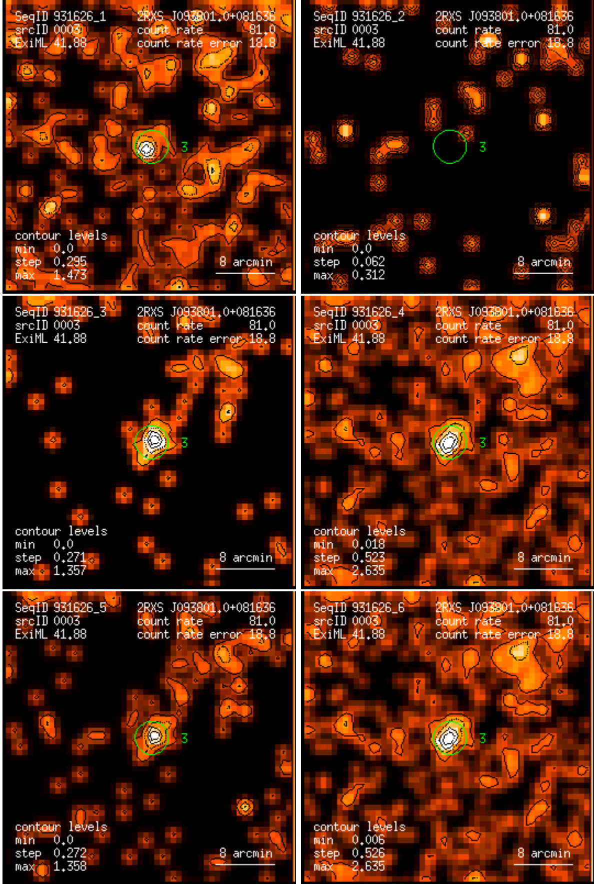
Figure 3: RASS 931626: detection 0003: band rate images, Gaussian filter: (1) PSPC channels 11 – 41, (2) 52 – 90, (3) 91 – 201, (4) 11 – 235, (5) 52 – 201, (6) 11 – 201. Broad band rates in counts/ks. Band rate contour levels in counts/ks/arcmin 2 .
