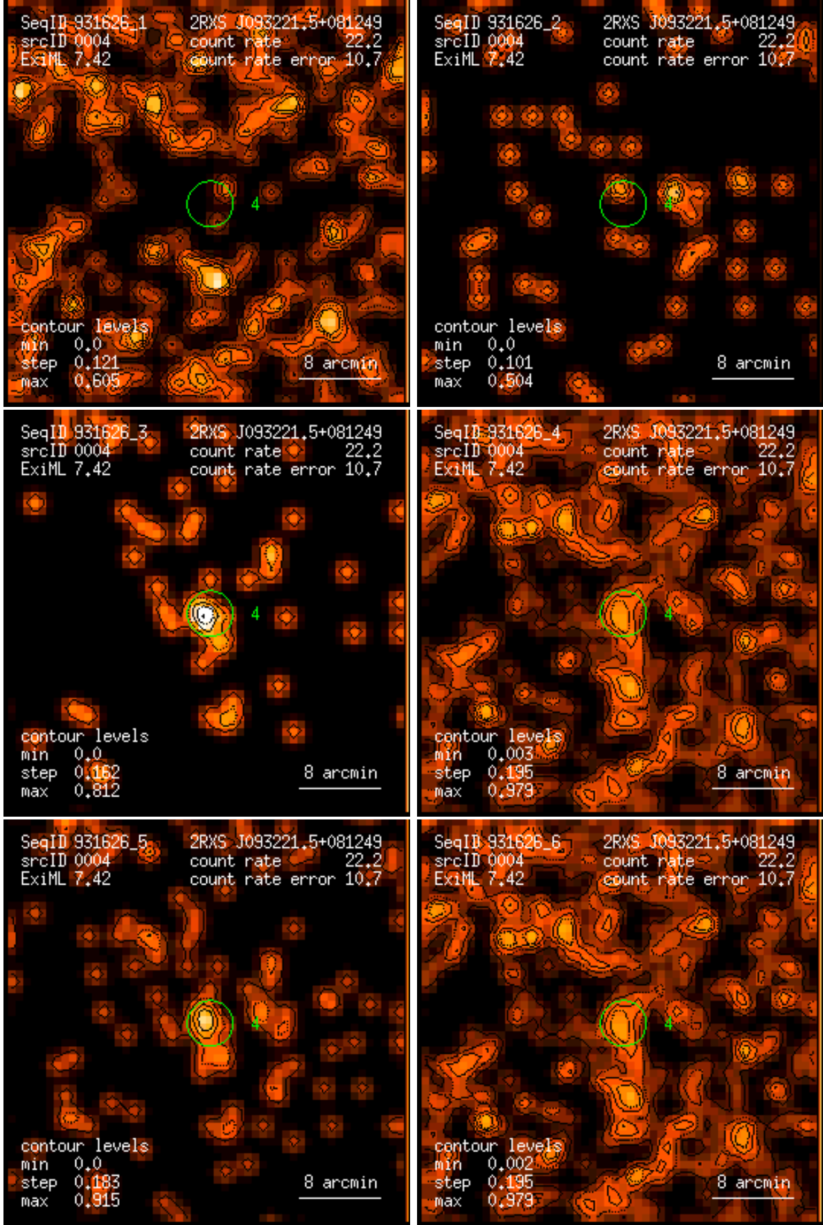
Figure 4: RASS 931626: detection 0004: band rate images, Gaussian filter: (1) PSPC channels 11 – 41, (2) 52 – 90, (3) 91 – 201, (4) 11 – 235, (5) 52 – 201, (6) 11 – 201. Broad band rates in counts/ks. Band rate contour levels in counts/ks/arcmin 2 .
