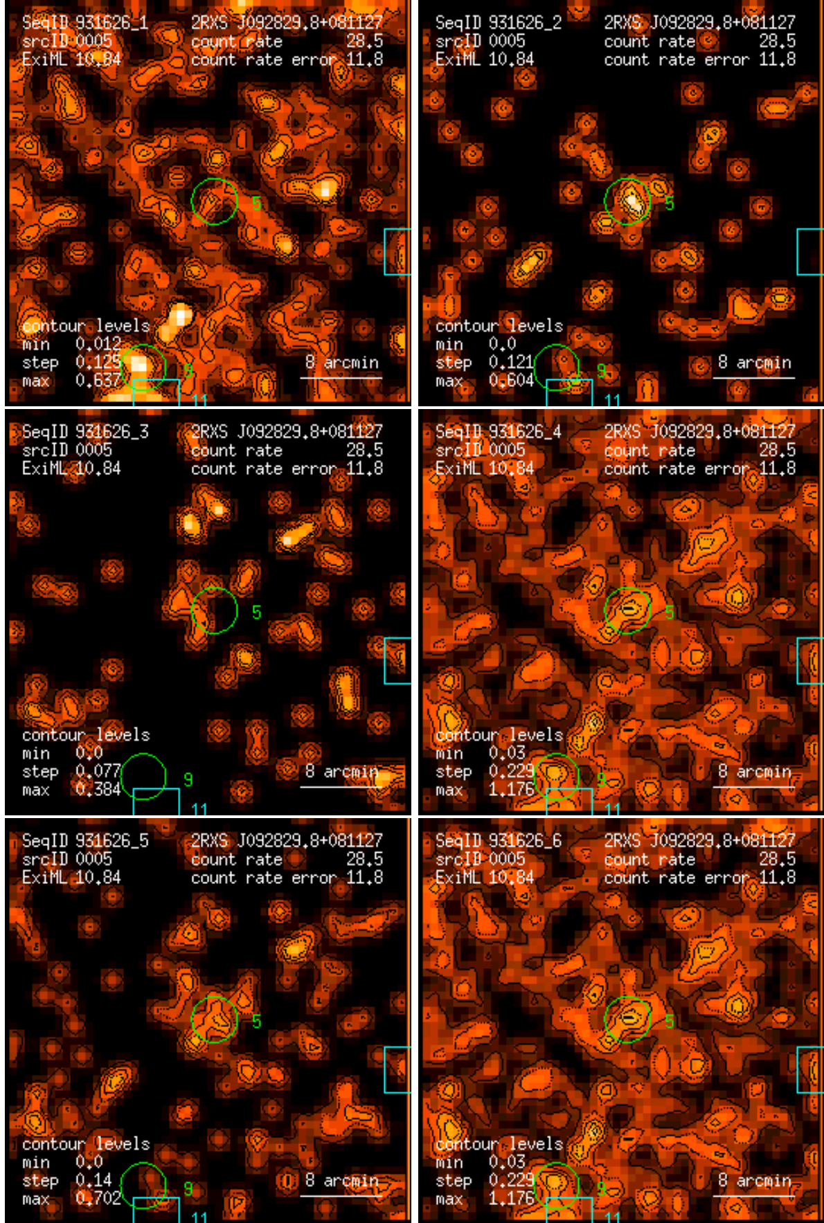
Figure 5: RASS 931626: detection 0005: band rate images, Gaussian filter: (1) PSPC channels 11 – 41, (2) 52 – 90, (3) 91 – 201, (4) 11 – 235, (5) 52 – 201, (6) 11 – 201. Broad band rates in counts/ks. Band rate contour levels in counts/ks/arcmin 2 .
