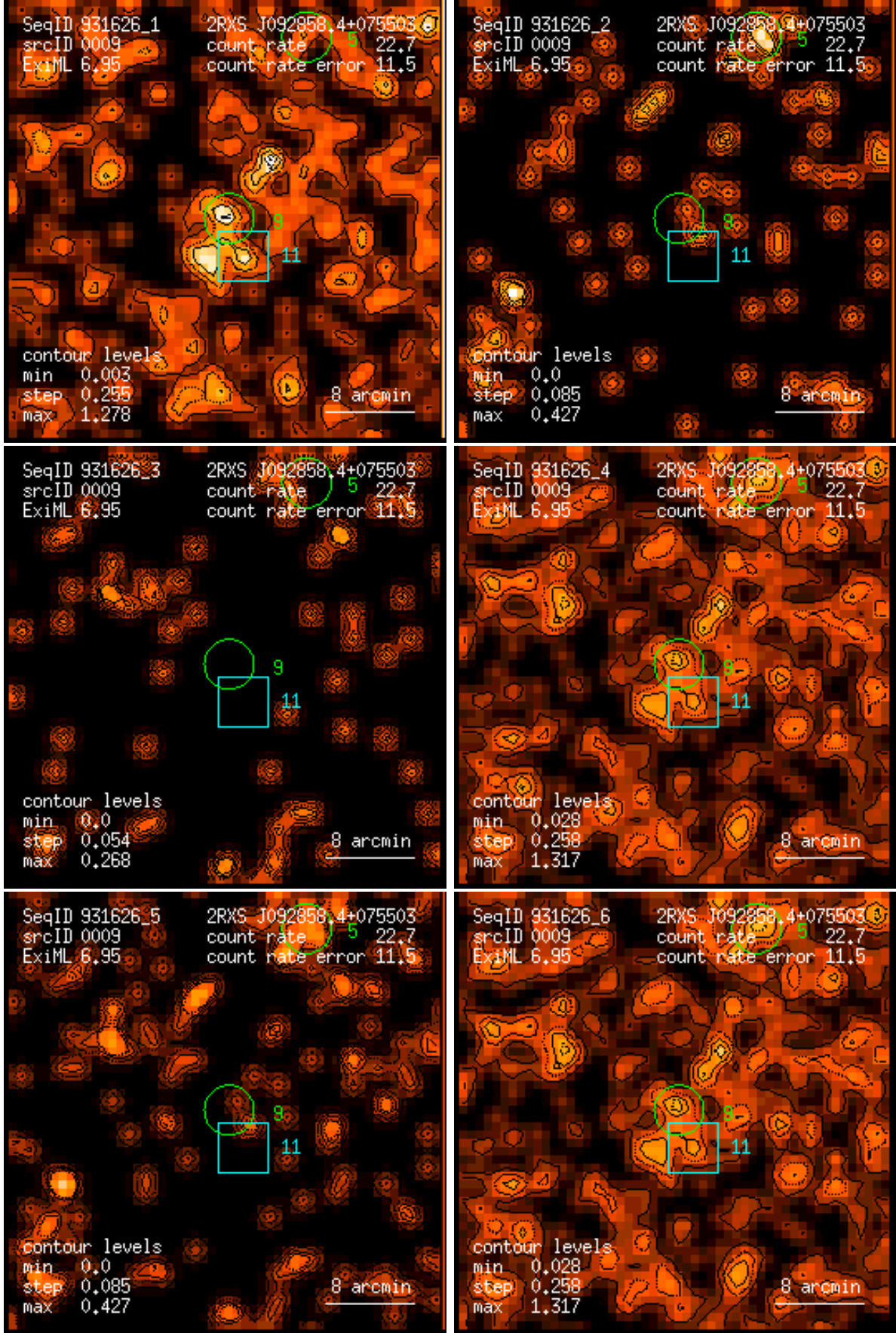
Figure 9: RASS 931626: detection 0009: band rate images, Gaussian filter: (1) PSPC channels 11 – 41, (2) 52 – 90, (3) 91 – 201, (4) 11 – 235, (5) 52 – 201, (6) 11 – 201. Broad band rates in counts/ks. Band rate contour levels in counts/ks/arcmin 2 .
