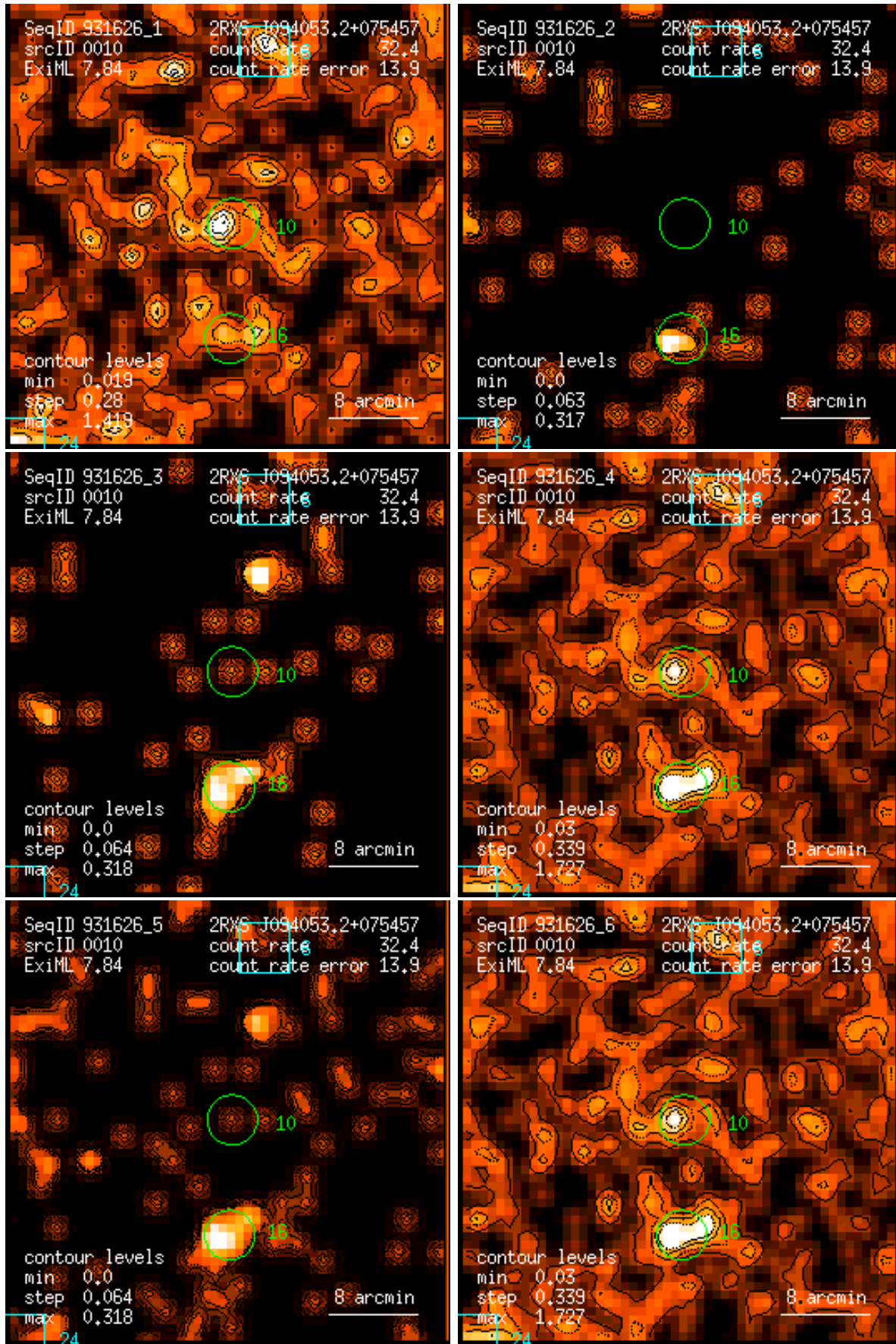
Figure 10: RASS 931626: detection 0010: band rate images, Gaussian filter: (1) PSPC channels 11 – 41, (2) 52 – 90, (3) 91 – 201, (4) 11 – 235, (5) 52 – 201, (6) 11 – 201. Broad band rates in counts/ks. Band rate contour levels in counts/ks/arcmin 2 .
