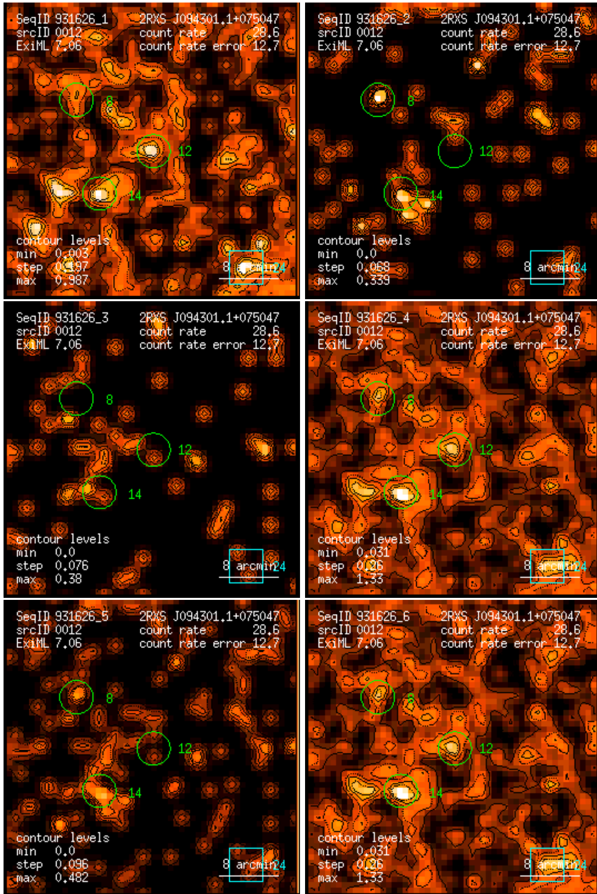
Figure 12: RASS 931626: detection 0012: band rate images, Gaussian filter: (1) PSPC channels 11 – 41, (2) 52 – 90, (3) 91 – 201, (4) 11 – 235, (5) 52 – 201, (6) 11 – 201. Broad band rates in counts/ks. Band rate contour levels in counts/ks/arcmin 2 .
