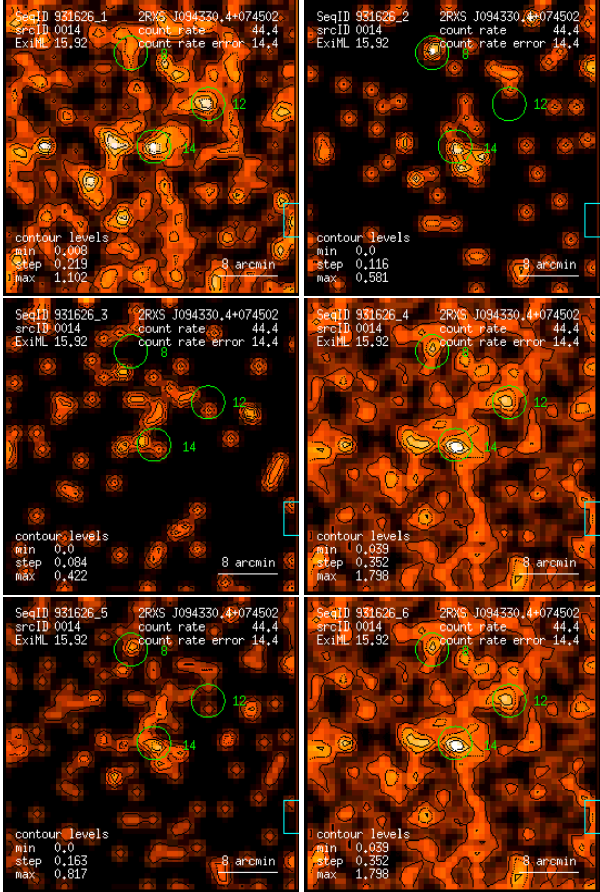
Figure 14: RASS 931626: detection 0014: band rate images, Gaussian filter: (1) PSPC channels 11 – 41, (2) 52 – 90, (3) 91 – 201, (4) 11 – 235, (5) 52 – 201, (6) 11 – 201. Broad band rates in counts/ks. Band rate contour levels in counts/ks/arcmin 2 .
