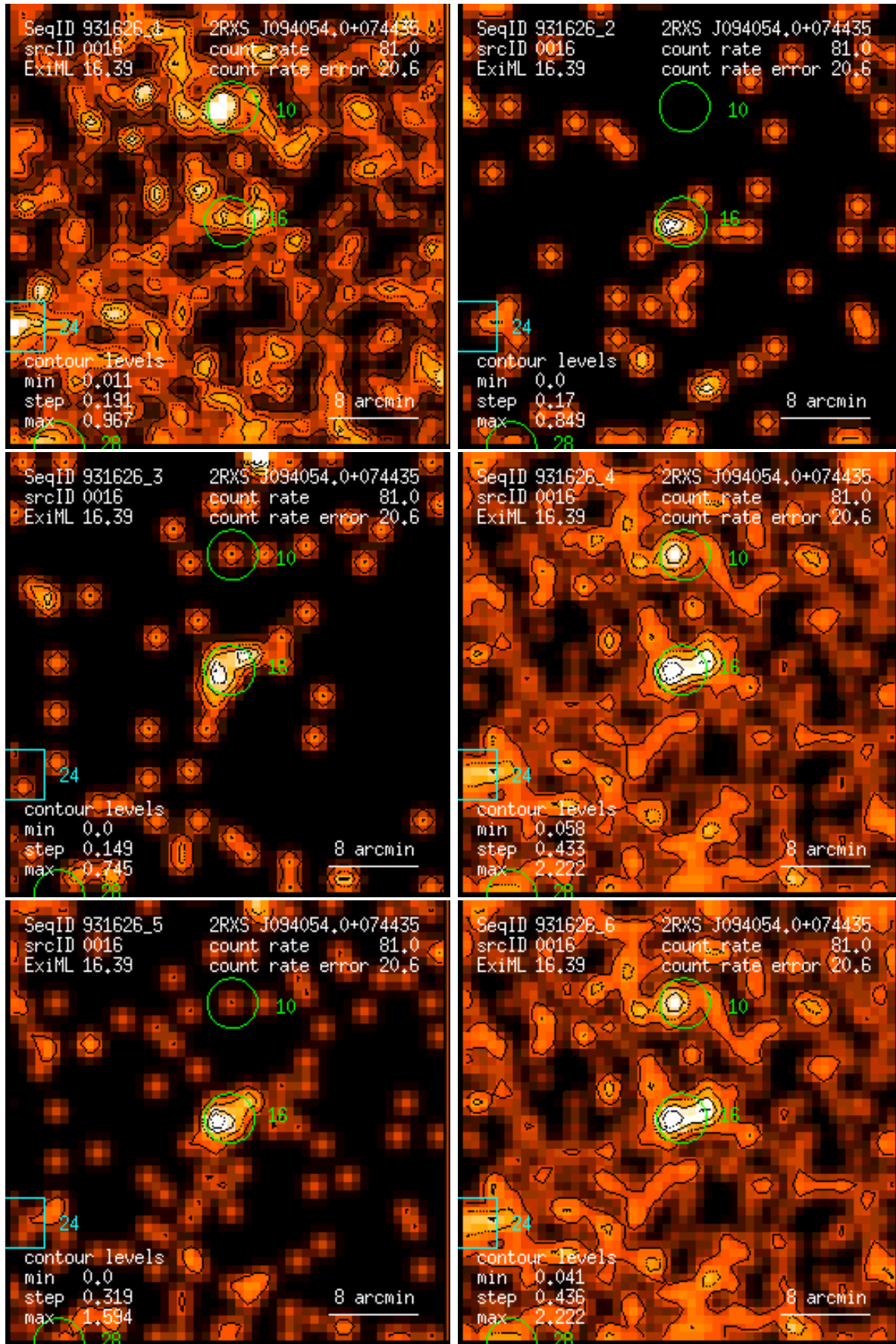
Figure 16: RASS 931626: detection 0016: band rate images, Gaussian filter: (1) PSPC channels 11 – 41, (2) 52 – 90, (3) 91 – 201, (4) 11 – 235, (5) 52 – 201, (6) 11 – 201. Broad band rates in counts/ks. Band rate contour levels in counts/ks/arcmin 2 .
