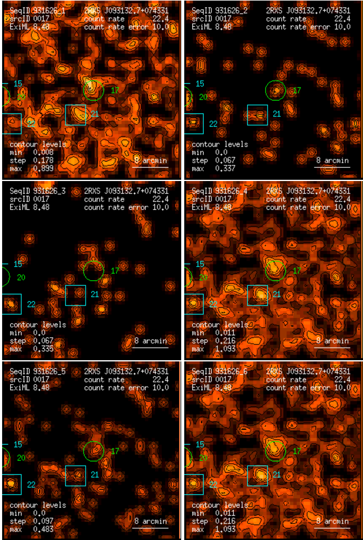
Figure 17: RASS 931626: detection 0017: band rate images, Gaussian filter: (1) PSPC channels 11 – 41, (2) 52 – 90, (3) 91 – 201, (4) 11 – 235, (5) 52 – 201, (6) 11 – 201. Broad band rates in counts/ks. Band rate contour levels in counts/ks/arcmin 2 .
