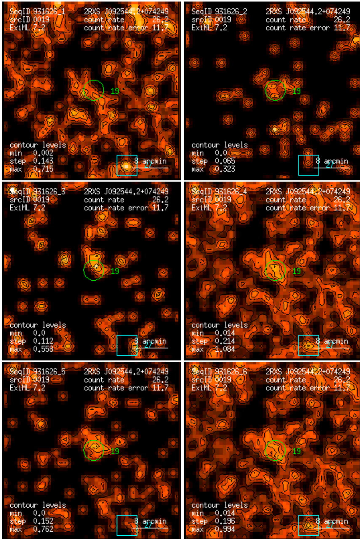
Figure 19: RASS 931626: detection 0019: band rate images, Gaussian filter: (1) PSPC channels 11 – 41, (2) 52 – 90, (3) 91 – 201, (4) 11 – 235, (5) 52 – 201, (6) 11 – 201. Broad band rates in counts/ks. Band rate contour levels in counts/ks/arcmin 2 .
